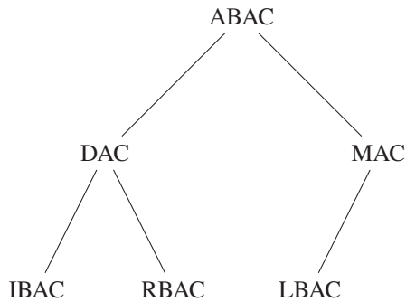
Figure 1. Non-Exhaustive Access Control Model Hierarchy
