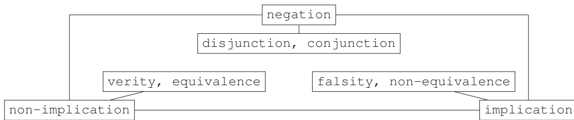
Figure 2. Wernick's Functionally Complete Two-Function Sets [18]
