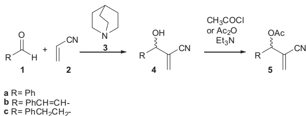
Scheme 2. Preparation of Morita-Baylis-Hillman adducts 4 and acetates 5 .
