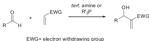
Scheme 1. Morita-Baylis-Hillman reaction.
