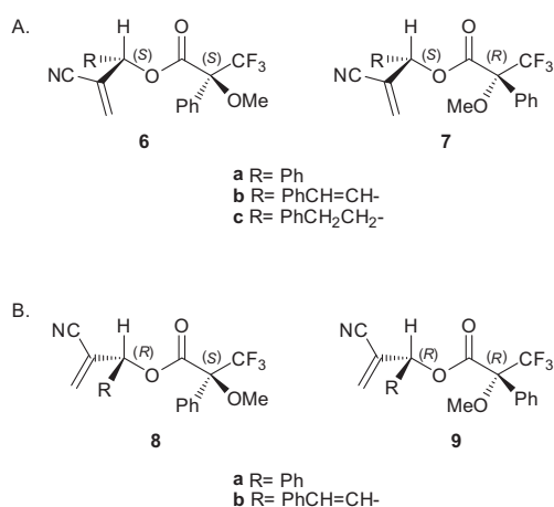
Figure 1. ( S )- and ( R )-Mosher ester derivatives: A. 6a–c and 7a–c ; B. 8a–b and 9a–b .
