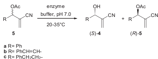
Scheme 3. Enzymatic hydrolysis of Morita-Baylis-Hillman acetates 5 .
