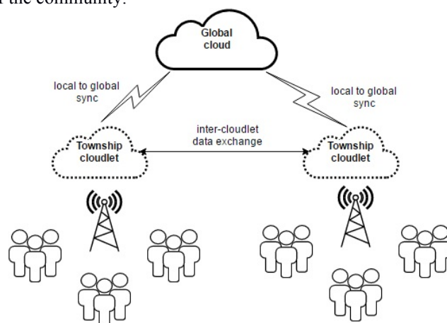
Figure 1. Cloudlet infrastructure
