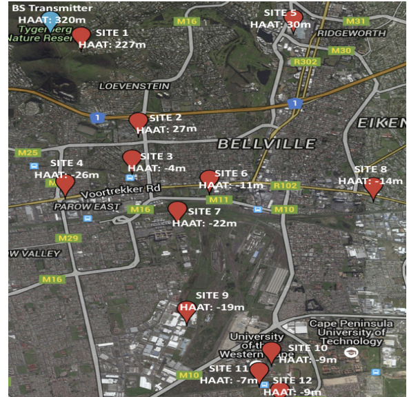
Figure 3: Measurement sites relative to BS transmitter
