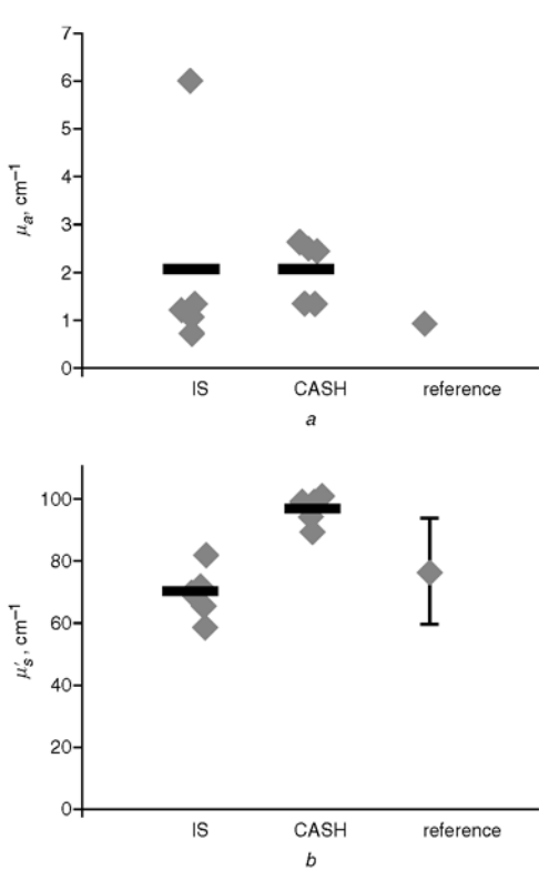
Fig. 9 Results from measurements on white matter at 633 nm performed with IS and CASH sensor. Published data for human brain are denoted reference (error bars indicate variation of results obtained in published data; these variations are not visible in 9(a)). (a) Absorption coefficient measurements; (b) reduced scattering coefficient measurements
