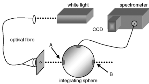
Fig. 2 Integrating sphere set-up. A and B are sample positions for measurements of T and R , respectively
