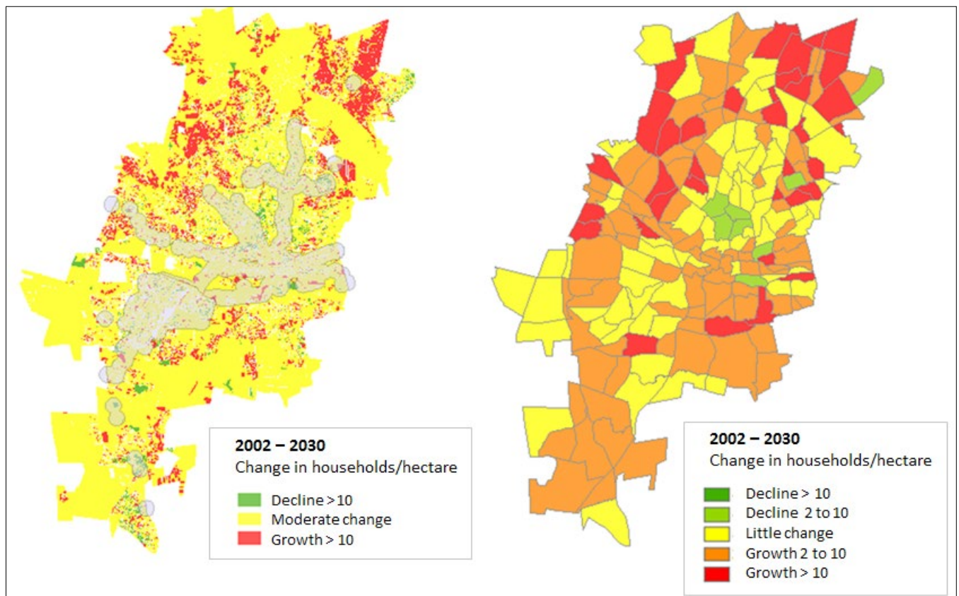
Figure 2: Projected change in population density in the City of Johannesburg between 2002 and 2030 at resolution of cadastral parcels (left) and Transport Analysis Zones (right)
