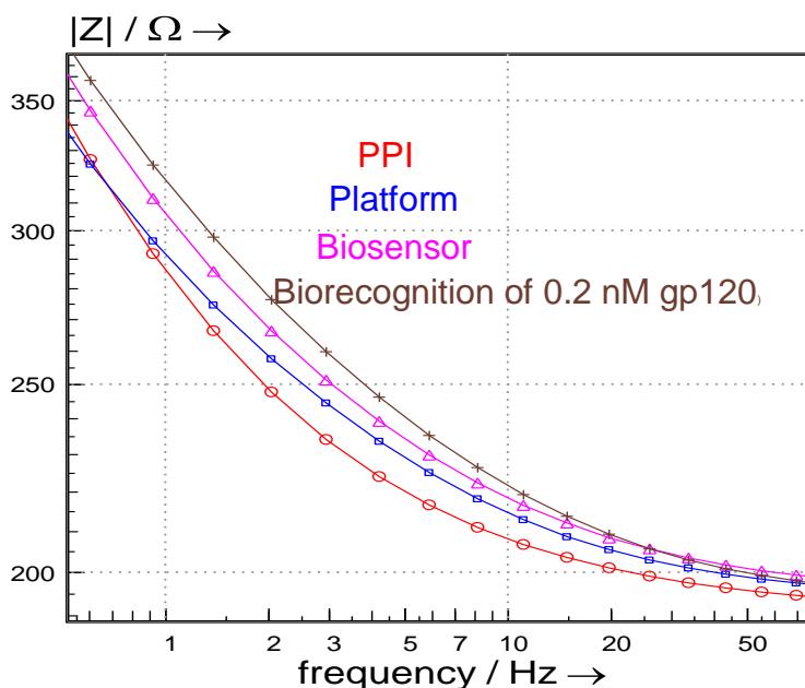
Figure 7. Impedance plots of biosensor fabrication and response to gp120 target in [\text{Fe}(\text{CN})_6]^{-3/4} redox probe.
