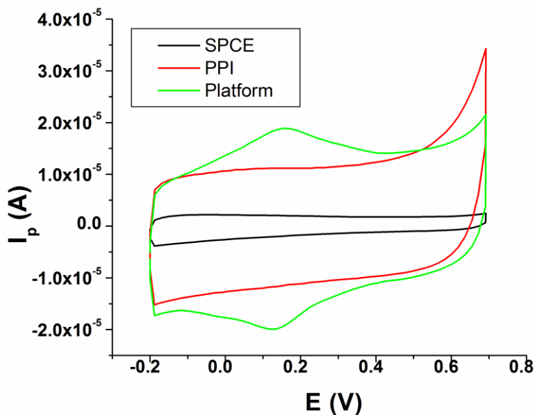
Figure 2. Cyclic voltammogram showing the bare SPCE, G4 PPI modified SPCE and G4 PPI-Strep platform in pH 7.5 PBS at scan rate 50 \text{ mV s}^{-1} .
