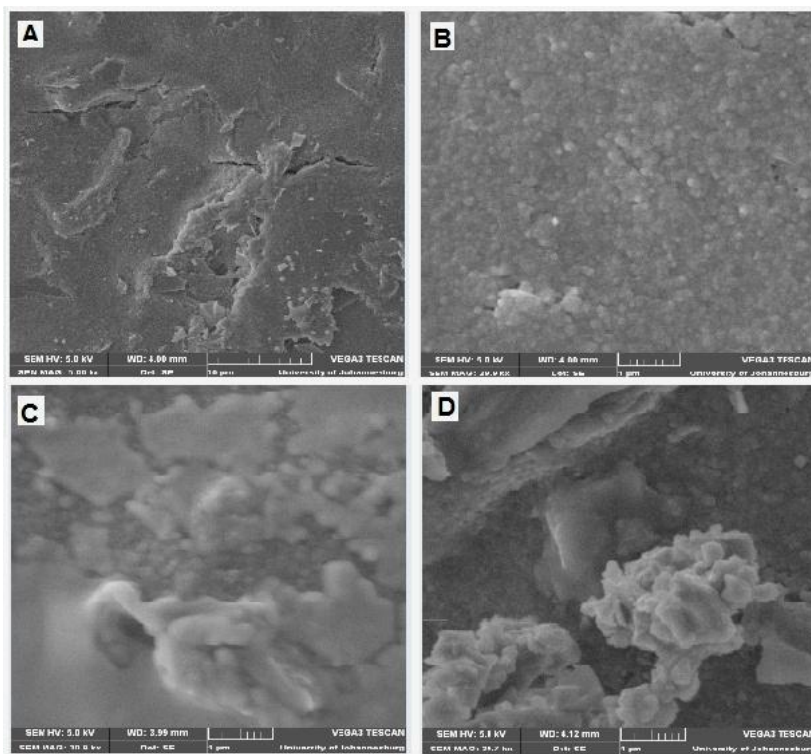
Figure 1. SEM (A) bare SPCE, (B) SPCE/PPI, (C) SPCE/PPI-Strep, (D) SPCE/Strep.
