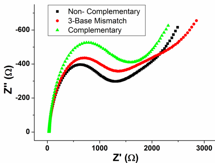
Figure 6. Nyquist plots of the impedance spectra of the DNA target hybridization in Fe(CN)_6^{3-/4-} showing selectivity of the sensor towards its complementary target.
