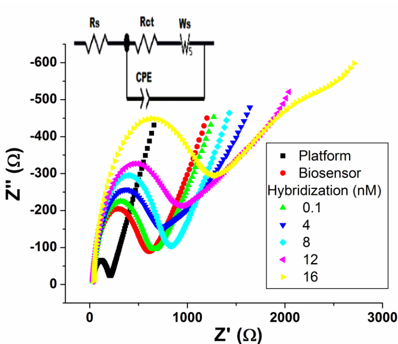
Figure 4. Nyquist plot showing the immobilization and hybridization process of GC/PPI/Strept modified electrode in Fe(CN)_6^{3-/4-} .
