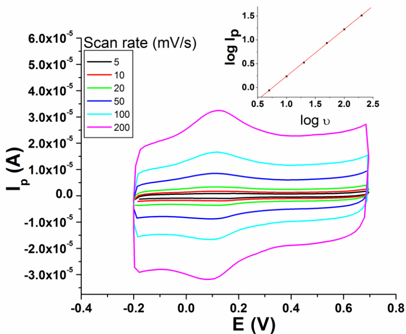
Figure 3. Scan rate study of SPCE/G4 PPI-Strep platform in PBS. Inset: log-log plot of I_p vs scan rate to test for surface adsorbed specie of the platform.
