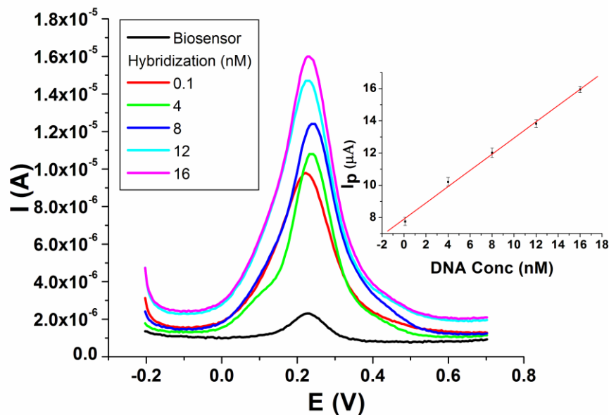
Figure 5. Square wave voltammetry of the immobilization and hybridization process in GC/G4 PPI/Strept modified electrode biosensor in pH 7.2 PB.
