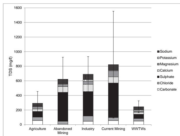
Figure 10 Mean total dissolved salt concentrations ( \pm standard deviation) and contribution of major ions to total TDS at once-off sampling sites representative of agriculture (n = 8), abandoned mining (n = 6), industry (n = 2), current mining (n = 10) and wastewater treatment works (n = 5) in the upper Olifants River catchment.
