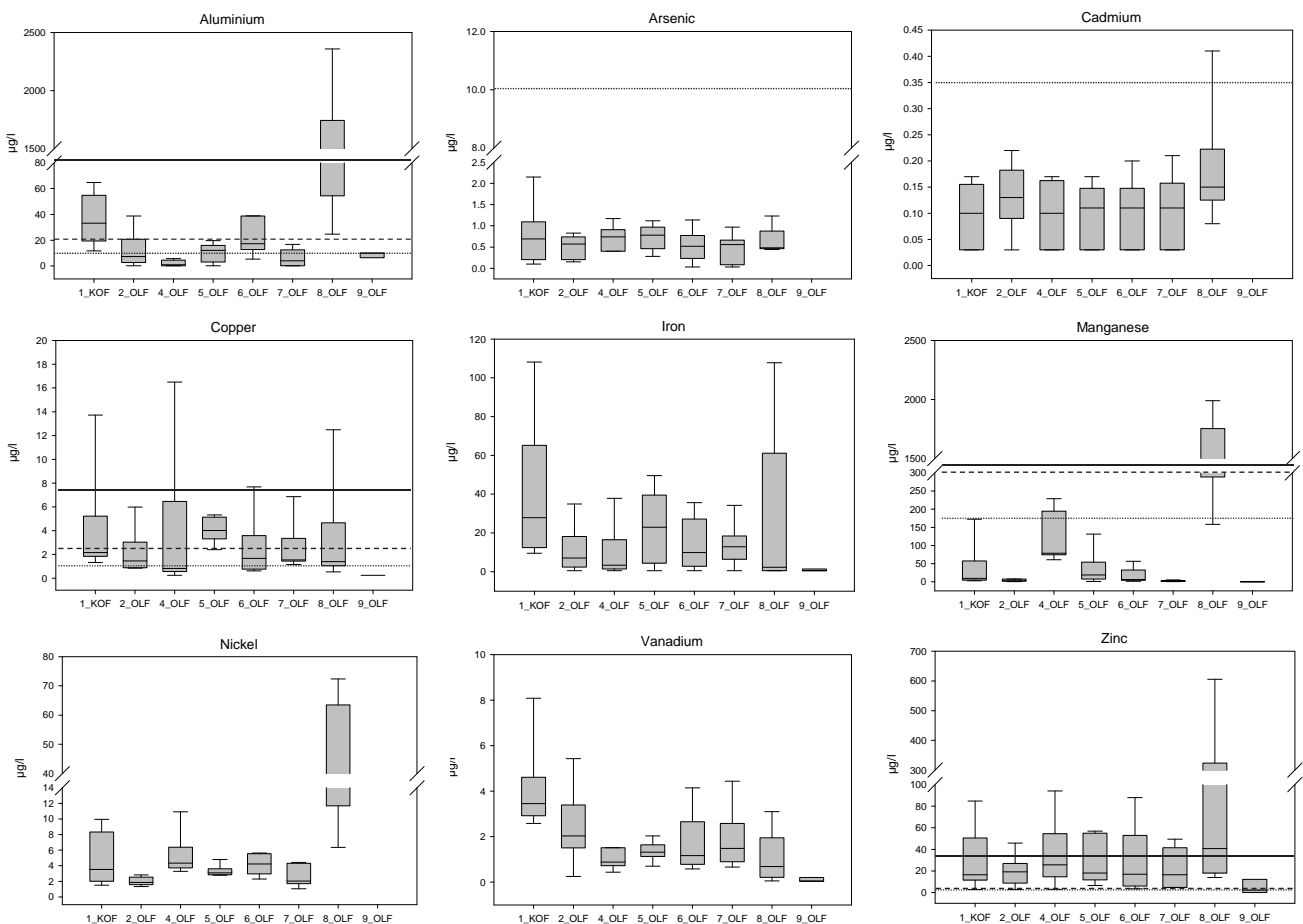
Figure 5 Box and whisker plots of metal concentrations measured at routine monitoring sites along the upper Olifants River ( n = 5 ). Dotted, dashed and solid lines represent the TWQR, CEV and AEV guideline values, respectively, as specified by DWAF (1996).
