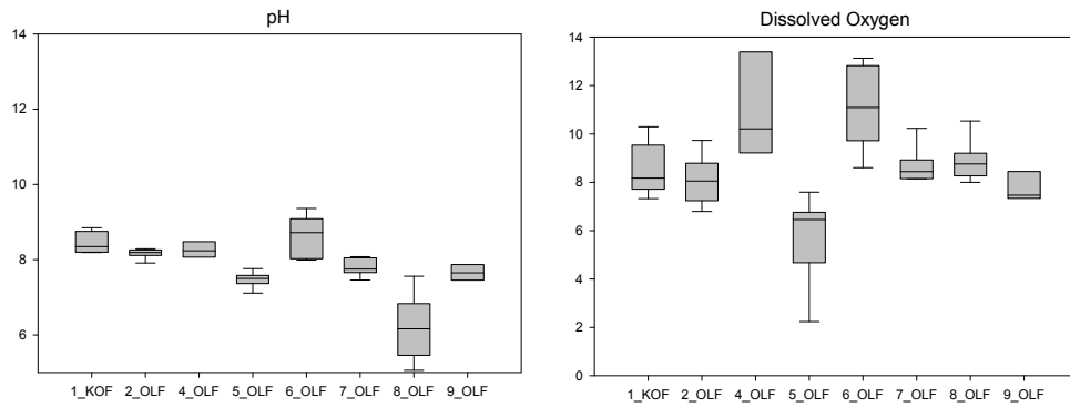
Figure 2 Box and whisker plots of pH and dissolved oxygen concentration (mg/l) measurements at routine monitoring sites along the upper Olifants River (n=5).
