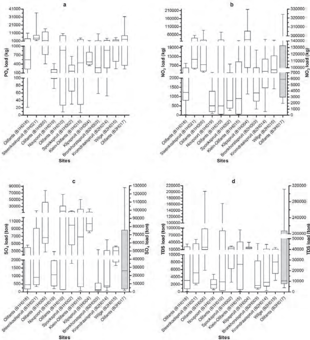
Figure 12 Minimum, 25 th , median, 75 th and maximum percentiles of annual phosphate, nitrate, sulphate and total dissolved solids loads measured at Department of Water Affairs monitoring sites located in the upper Olifants catchment from 2000 to 2010. Shaded bars are read on the right-hand y-axis
