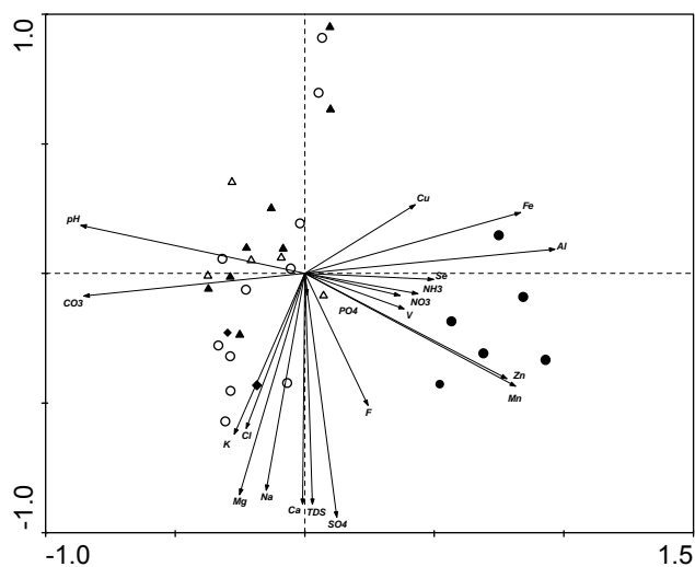
Figure 9 Principal component analysis (PCA) of measured water quality parameters (black arrows) and sampling sites downstream of agriculture (solid triangle), abandoned mining (solid circle), current mining (open circle), industry (solid diamond) and wastewater treatment works (open triangle) in the upper Olifants River catchment.
