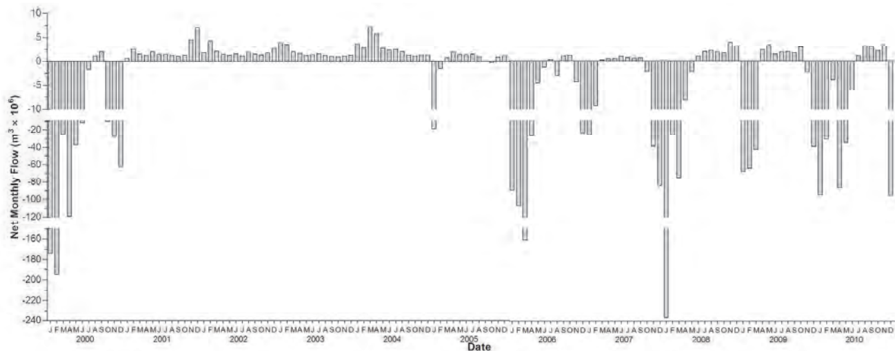
Figure 8 Net monthly flow originating from acidic streams (sum of Klipspruit and Spookspruit) versus alkaline rivers (sum of Olifants and Klein-Olifants). Positive values indicate a net acidic flow and negative values indicate a net alkaline flow.
