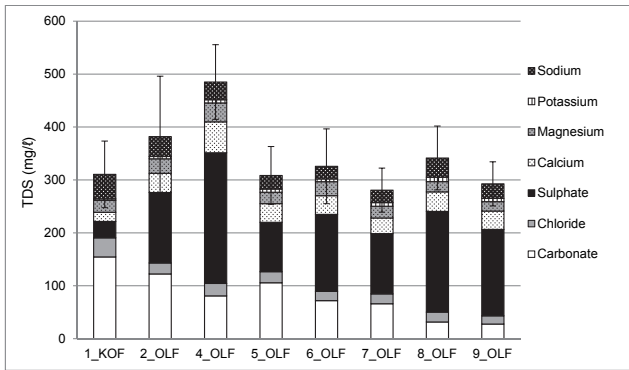
Figure 4 Mean ( n = 5 ) total dissolved salts (TDS) concentrations ( \pm standard deviation) and contribution of major ions to total TDS at routine sampling sites along the upper Olifants River.
