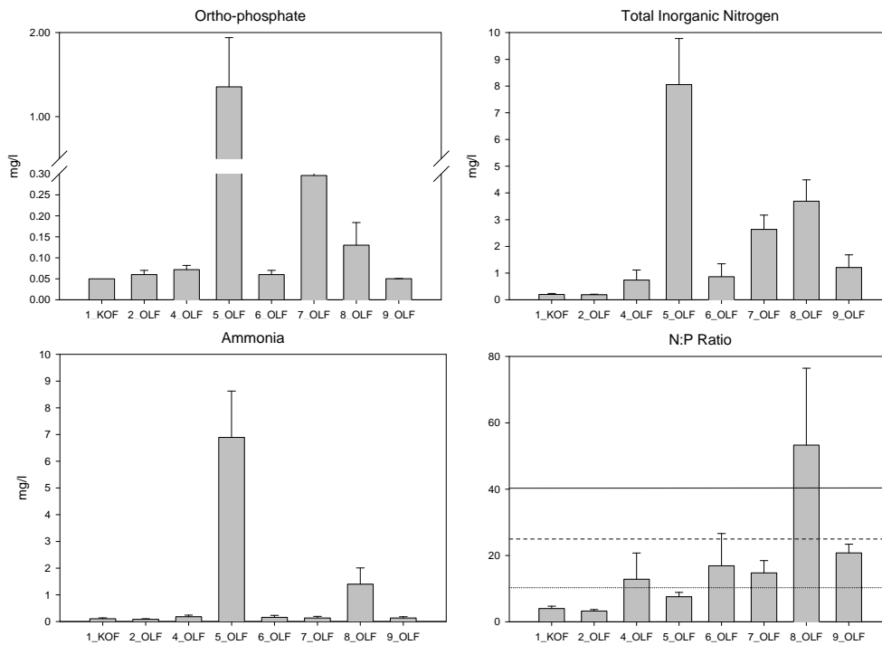
Figure 3 Mean concentrations (ortho-phosphate, total inorganic nitrogen and ammonia) and N:P ratios of nutrients measured at routine monitoring sites along the upper Olifants River (n=5). Solid, dashed and dotted lines are representative of eutrophic, mesotrophic and oligotrophic status, respectively.
