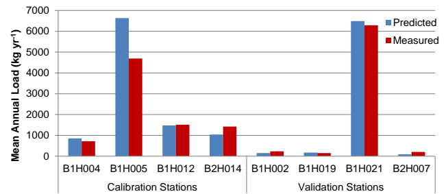
Figure 3. Predicted and observed mean annual ortho-phosphate loads at calibration and validation monitoring stations located in the upper Olifants catchment from 2002 to 2010.
