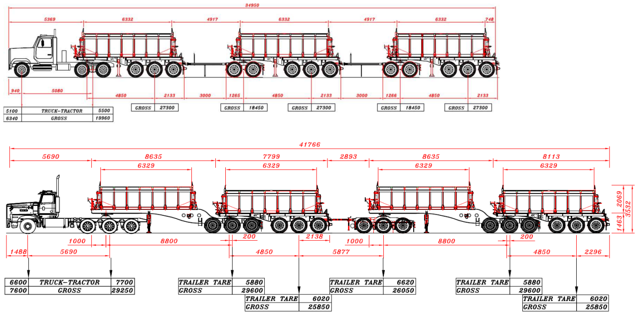
Figure 3-7 Unitrans Mining baseline and PBS road trains (Richards Bay Minerals mining operation)
