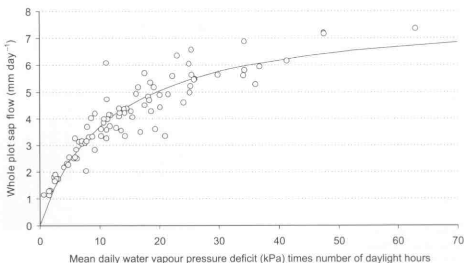
Fig. 1. The relation between whole-plot sap flow and the product of mean daily water vapour pressure deficit and the number of daylight hours, recorded in a riparian stand of black wattle in the Wellington district, Western Cape. 4
