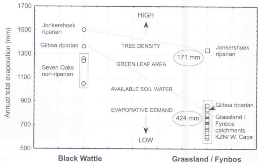
Fig. 7. A chart summarizing annual total evaporation estimated for black wattle and grassland/fynbos vegetation at various sites in KwaZulu-Natal and the Western Cape. The Jonkershoek and Gilboa black wattle estimates are based on model predictions. Major vegetation characteristics governing the net change in total evaporation (shown by the values in ovals) following invasion or clearance of black wattle in grassland and fynbos shrubland catchments are shown in the centre of the chart.
