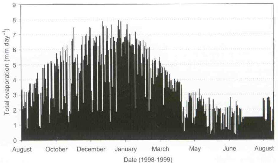
Fig. 5. The annual pattern of total evaporation from a riparian fynbos plant community in the Jonkershoek valley, Western Cape, for the period 26 August 1998 to 25 August 1999. A period of constant total evaporation contains patched data based on mean daily total evaporation on either side of the data gap. 4
