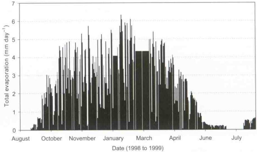
Fig. 4. Daily total evaporation from a seasonally wet grassland at Gilboa, KwaZulu-Natal Midlands, for the period 15 August 1998 to 31 August 1999. Two periods of constant total evaporation contain patched data based on mean daily total evaporation on either side of the data gap. 4
