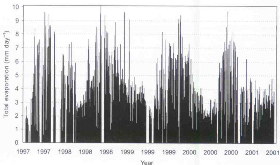
Fig. 2. Patterns of daily total evaporation recorded for a black wattle plantation in the Seven Oaks district, KwaZulu-Natal, for the period 1 August 1997 to 30 July 2001.
