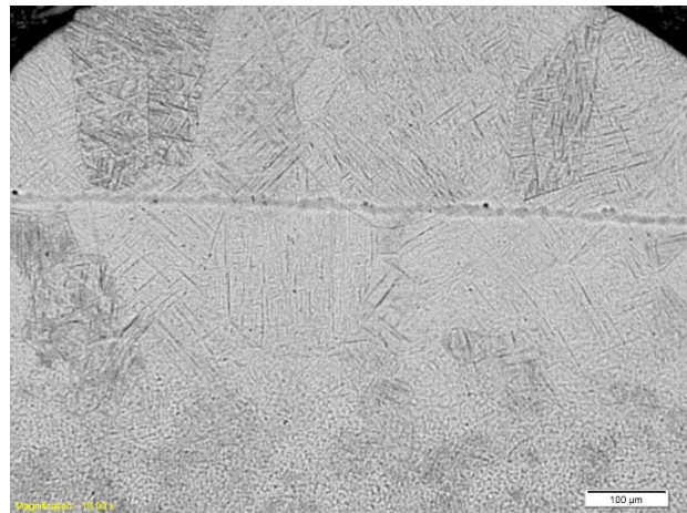
Figure 6: The micrograph of sample at a laser power of 400 W [10]
