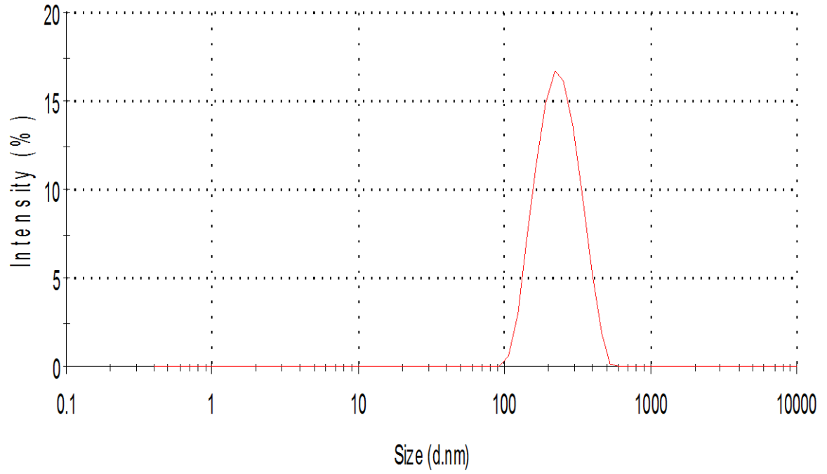
Fig.2 Particle size distributions by intensity as a function of particle size for PCL-EFV nanoparticles in water.
