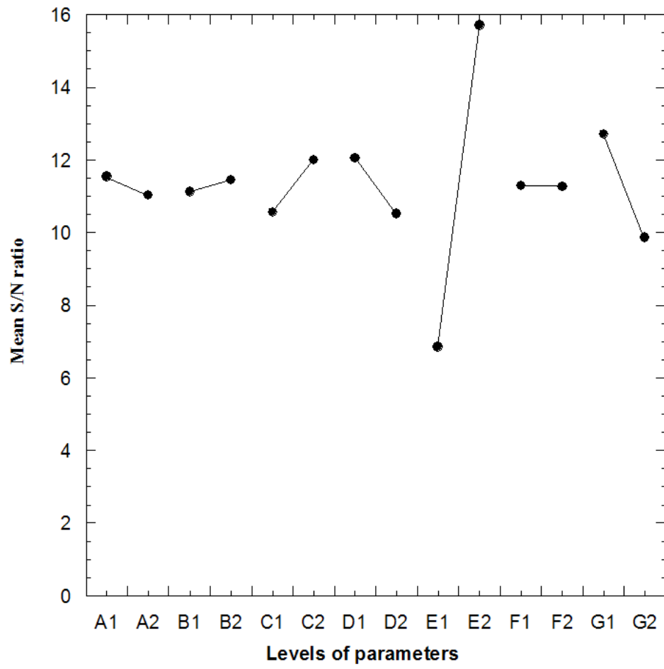
a) S/N graph for particle size
