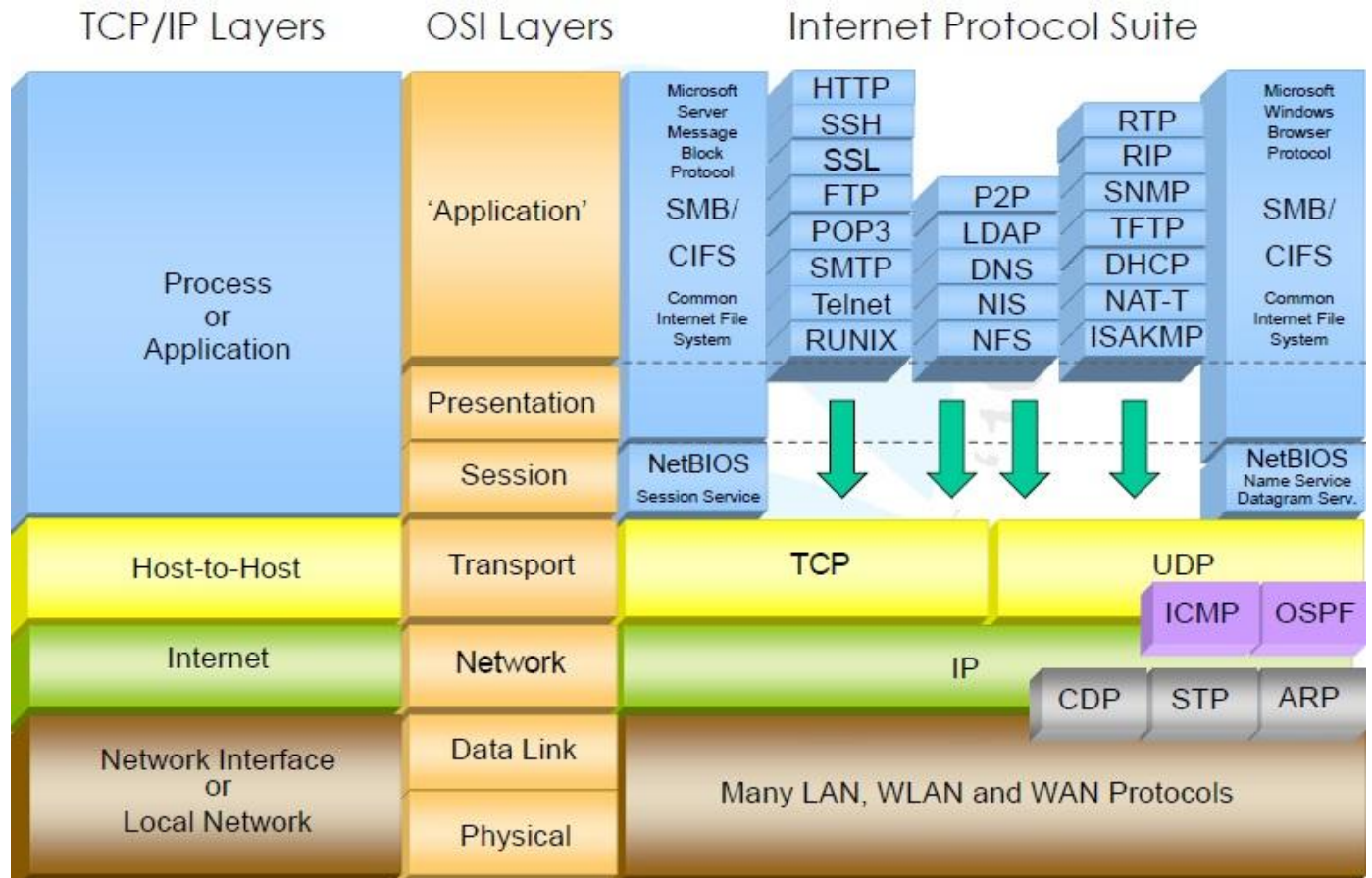
Figure 1 Open Systems Interconnection model (OSI model)[5]
