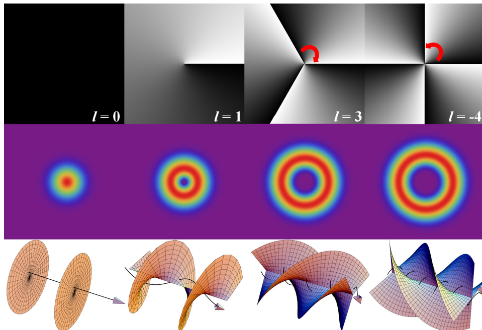
Fig. 1.5.4. Top row : Phase profiles for various vortex modes. The red arrow denotes the rotation in the phase profile. Middle row : Corresponding transverse intensity profiles for the various vortex modes. Bottom row : Corresponding wavefronts for the various vortex modes, courtesy of [36].
