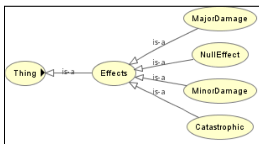
Figure 2: Effects Class
