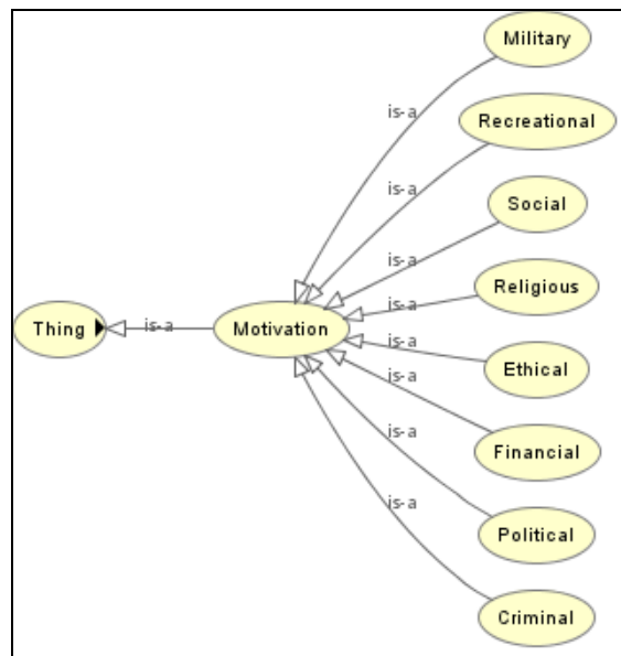
Figure 3: Motivation Class
