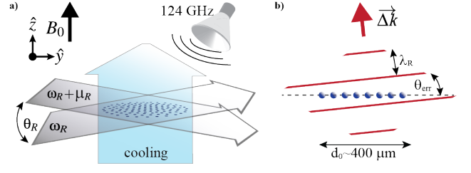
Figure 6. (a) Sketch of the ODF laser beam geometry used to generate the one dimensional (1D) traveling optical lattice. (b) Sketch of the 1D optical lattice wave fronts (red lines). These wave fronts need to be aligned with the ion planar array (represented by the blue dots). Here \lambda_R = 2\pi/|\delta\vec{k}| \approx 3.7 \mu\text{m} and \theta_{err} denotes the angle of misalignment. 400 \mu\text{m} is the typical array diameter for N \sim 200 ions. With the wavefront alignment technique discussed in the text we obtain \theta_{err} < 0.05^\circ .
