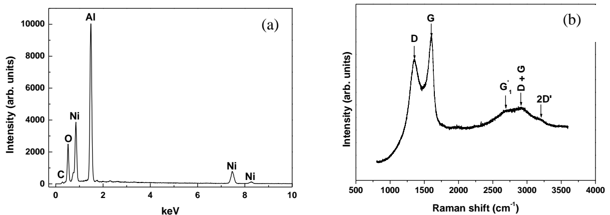
Fig. 4. (a) A typical EDS spectrum for C/NiO nanocomposite coated on aluminum substrate, (b) Raman spectra of the C/NiO nanocomposite coating.
