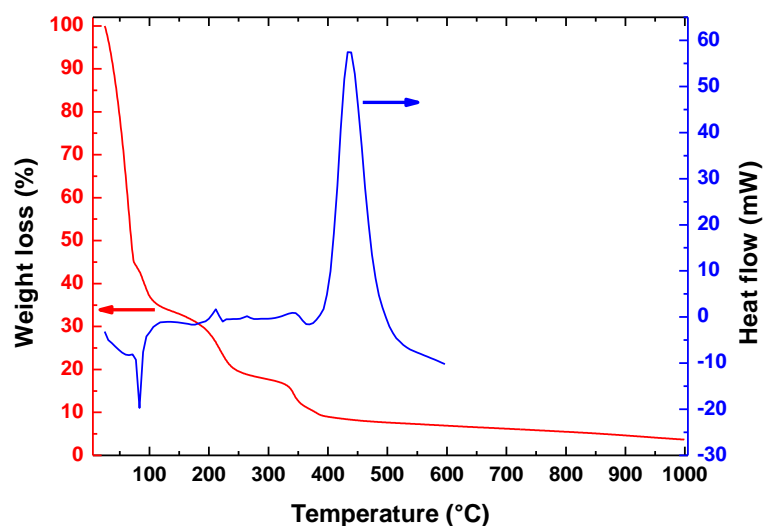
Fig. 2. Typical TGA and DSC spectra for C/NiO precursor solution.
