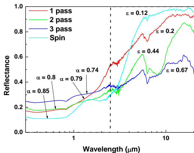
Fig. 5. The near normal reflectance spectra of C/NiO nanocomposite deposited with different passes on aluminum substrate etched with \text{H}_3\text{PO}_4 . The spectrum for spin coated samples is also included for comparison. The broken line represents the reflectance spectrum for an ideal selective solar absorber.
