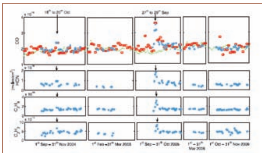
FIGURE 6 CO (top), HCN, C 2 H 6 (in middle) and C 2 H 2 (down) are trace gases simultaneously retrieved from FTIR data measured at Paramaribo in Suriname (lat 5.8°N, Long. 58.2°W)
