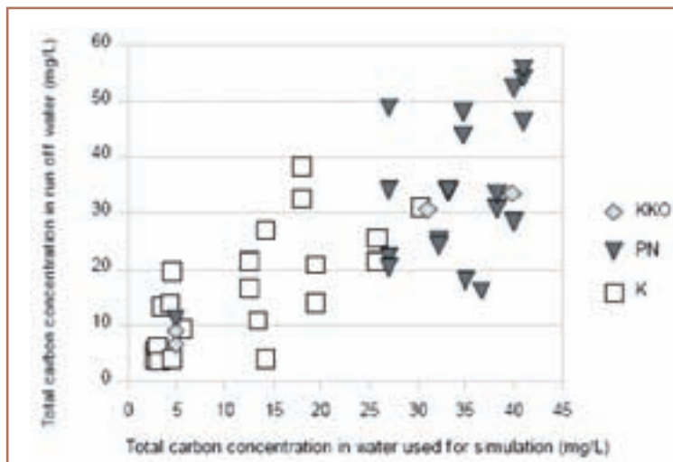
FIGURE 6 Carbon concentration in run off solutions and in the water used in the rainfall simulator. Influence of the water origin
