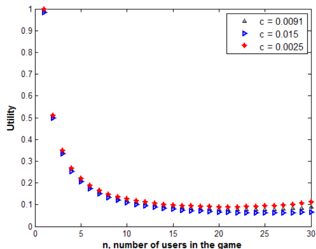
Figure 4: User Utilities with transmission cost, c
