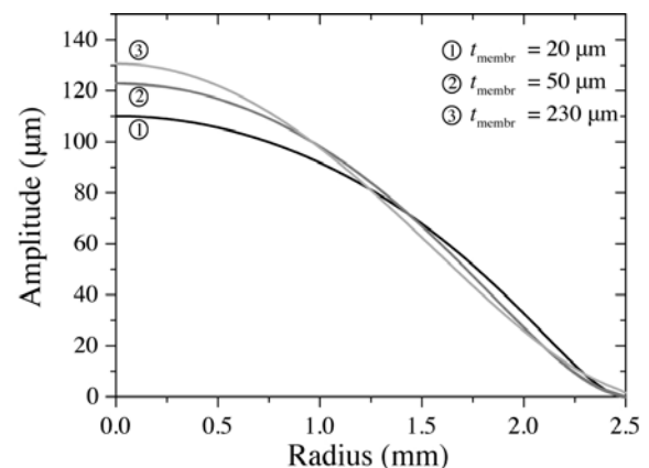
Figure 12: Simulated membrane shapes for a lens volume of 1 \mu\text{l} at divorce homogeneous membrane thicknesses.
