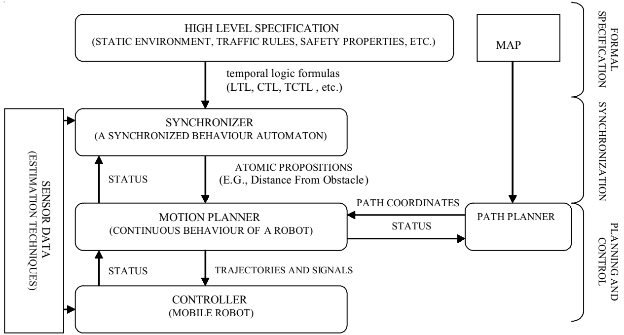
Figure 3. A proposed framework of a symbolic motion planning.
