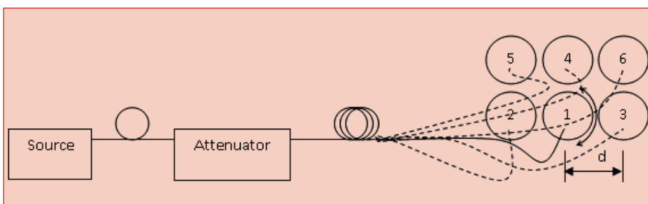
Fig. 3: Optical head positions and rotation to emulate the effect of fibre flexing during typical fibre optic power meter calibrations.
