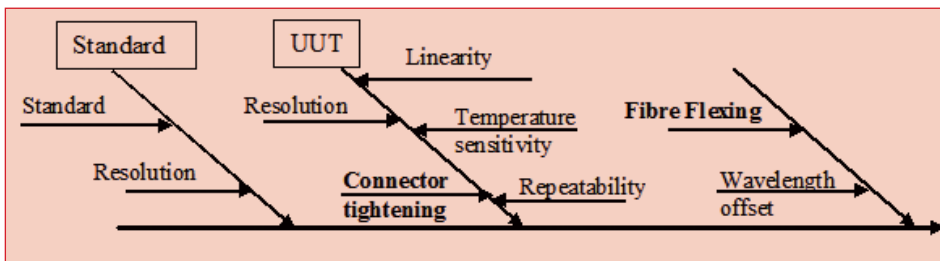
Fig. 2: Fishbone diagram of the uncertainty contributors.
