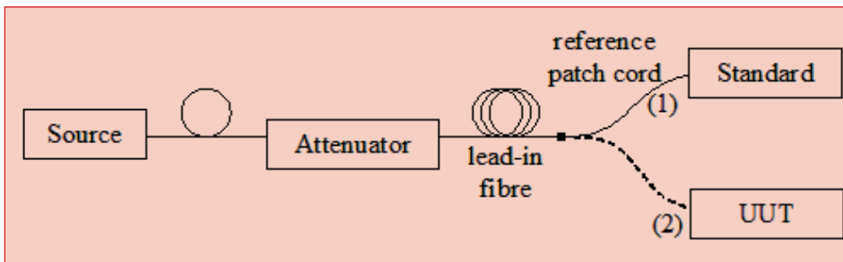
Fig. 1: Measurement setup for the calibration of an optical power meter/photodiode.
