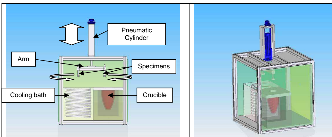
Figure 3: Aluminium Melt Cyclic Dipping Test Rig
