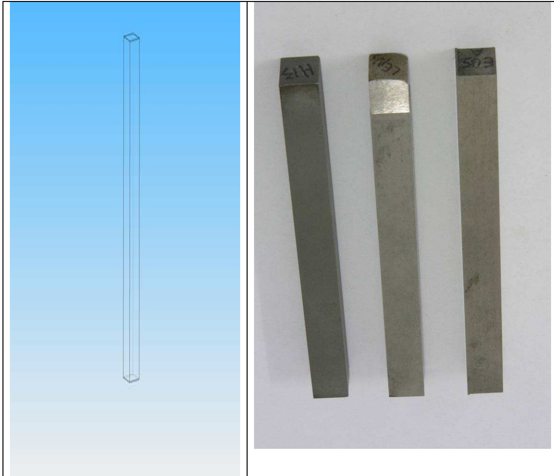
Figure 1: 3D model of the specimens, and the grown and machined specimens
