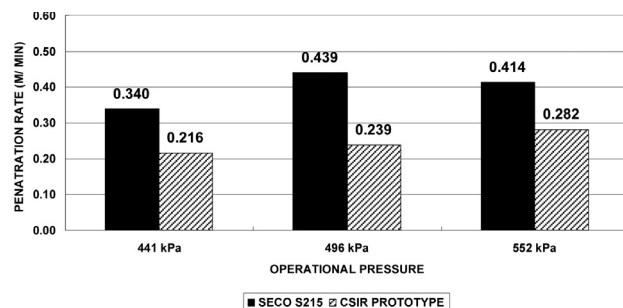
Figure 6—Performance comparisons while drilling in concrete
