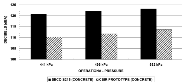
Figure 5—Sound power comparisons while drilling in concrete
