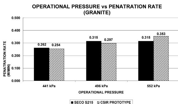
Figure 8—Performance comparisons while drilling in granite
