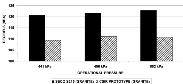
Figure 7—Sound power comparisons while drilling in granite
