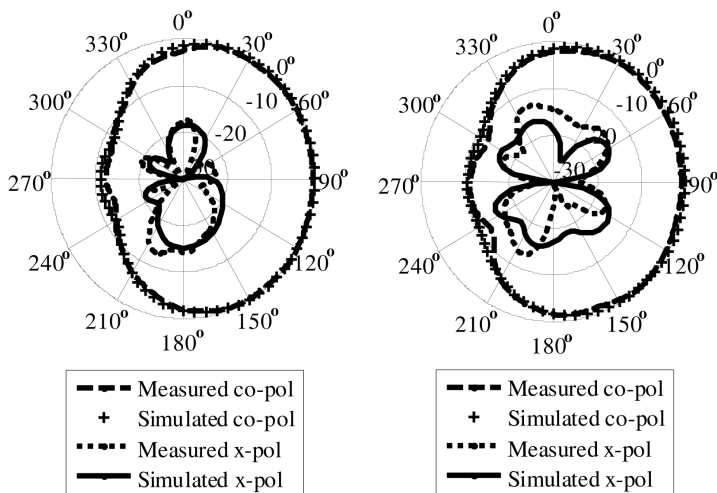
Figure 11. The measured and simulated normalized radiation pattern (as function of \varphi , \theta = 90^\circ , with reference to the coordinate system in Fig. 2) at 2.44 GHz in the H -plane. (a) Horizontal polarization. (b) Vertical polarization.
