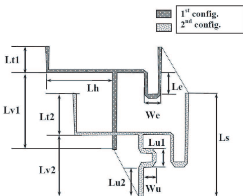
Figure 3. The two feeding configurations showing the design parameters.
