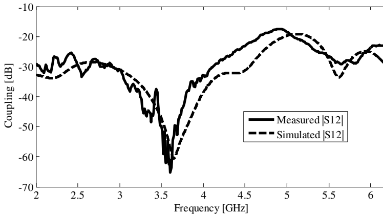
Figure 6. The coupling between Port 1 and Port 2.
