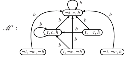
Figure 5: The result of revising model \mathcal{M} in Figure 2 by the new executability law \neg\text{token} \rightarrow \langle \text{buy} \rangle \top .
