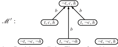
Figure 4: Revising \mathcal{M} in Figure 2 with \text{token} \rightarrow [\text{buy}]\neg\text{token} .
