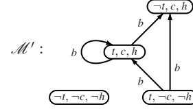
Figure 3: Revising model \mathcal{M} in Figure 2 with coffee \leftrightarrow hot .
