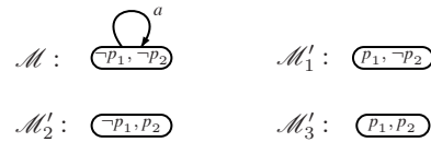
Figure 6: Model \mathcal{M} of \mathcal{T}_1 and revision of \mathcal{M} by p_1 \vee p_2 .
