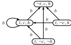
Figure 1: A transition system depicting the agent's knowledge about the dynamics of the coffee machine. b , t , c , and h stand for, respectively, buy , token , coffee , and hot .
