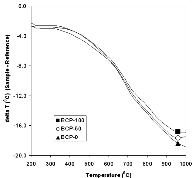
Fig. 12 SDTA measurements for BCP-0, 50 and 100, where \Delta T is the sample temperature minus the reference temperature
