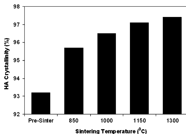
Fig. 3 Crystallinity of the solid state reaction-produced HA after sintering
