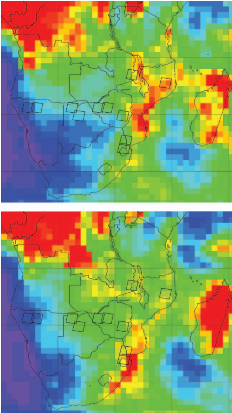
Figure 3. Eleven Landsat ETM+ validation scenes (black squares) superimposed upon annual precipitation estimates for 1999 (top) and 2000 (bottom). The annual precipitation estimates derived from the monthly 1^\circ Tropical Rainfall Measuring Mission best-estimate precipitation rate product (Huffman et al. 1995) (blue <300 mm, yellow >1000 mm, red >1500 mm). Country boundaries and meridians ( 10^\circ , 20^\circ , 30^\circ , 40^\circ , 50^\circ E) and parallels ( 10^\circ , 20^\circ , 30^\circ S) are shown (black lines).
