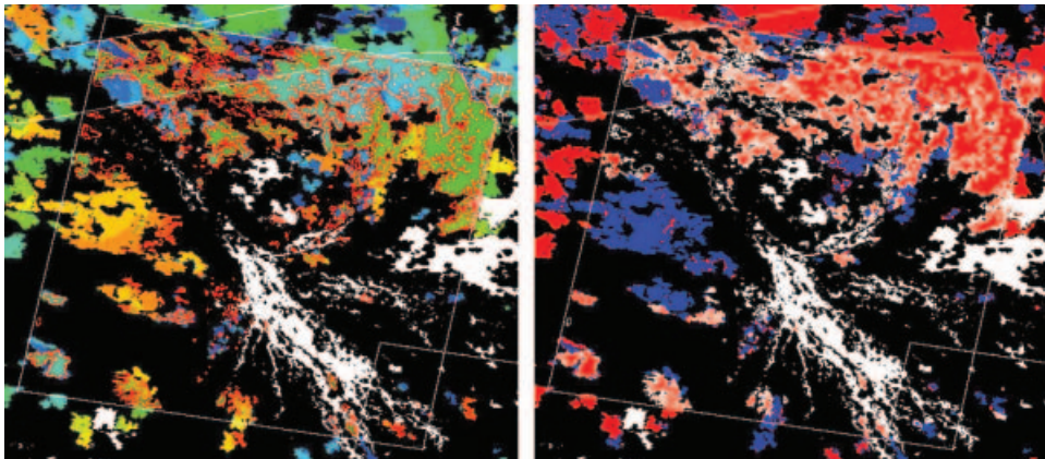
Figure 8. MODIS 500 m burned-area product and Landsat ETM+ independent burned area validation data, Okavango delta, Botswana (Landsat Path 175, Row 73, the north-west Botswana Landsat scene in figures 2 and 3). The vectors show independent burned area data mapped using the protocol from ETM+ acquisitions sensed 19 August, 4 September and 6 October 2001 (left: red vectors; right: white vectors). The MODIS burned areas are coloured in the same way as in figure 7. The 185 km \times 170 km Landsat ETM+ scene boundary and the Botswana, Namibia (Caprivi Strip) and Angola boundaries are also shown (white vectors, left and right).
