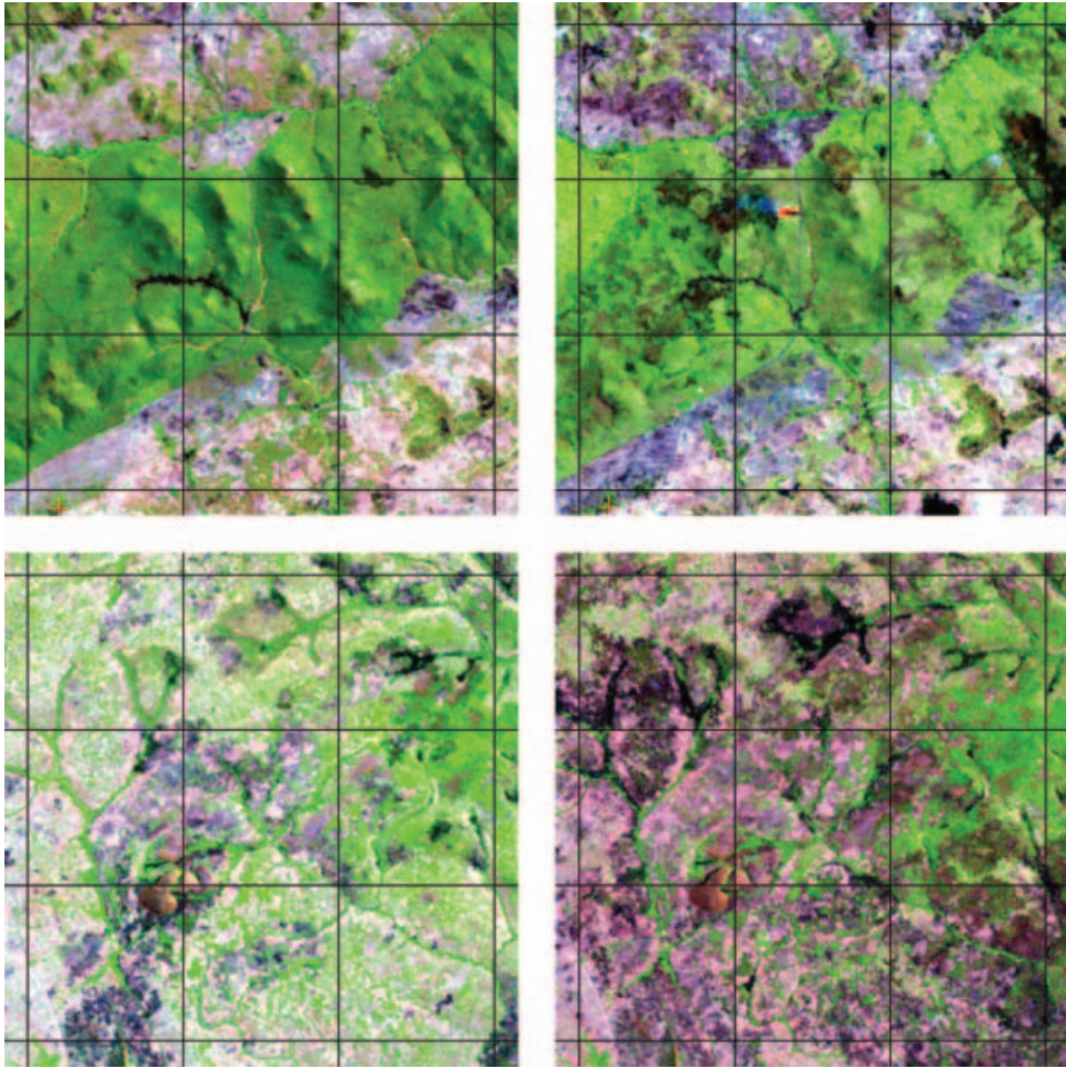
Figure 10. Landsat ETM+ subsets to illustrate regions that are difficult to map burned areas. Landsat ETM+ 30 m reflective wavelength data displayed as Red: band 5 (1550–1750 nm), Green: band 4 (750–900 nm), Blue: band 3 (630–690 nm). The top two images show spatial subsets over Chimaliro Forest Reserve, Malawi (left: 25 August; right: 26 September 2001). The bottom two images show spatial subsets over Mecuburi Forest Reserve, Mozambique (left: 14 September; right: 30 September 2001). The black grid lines are spaced every 3 km.
