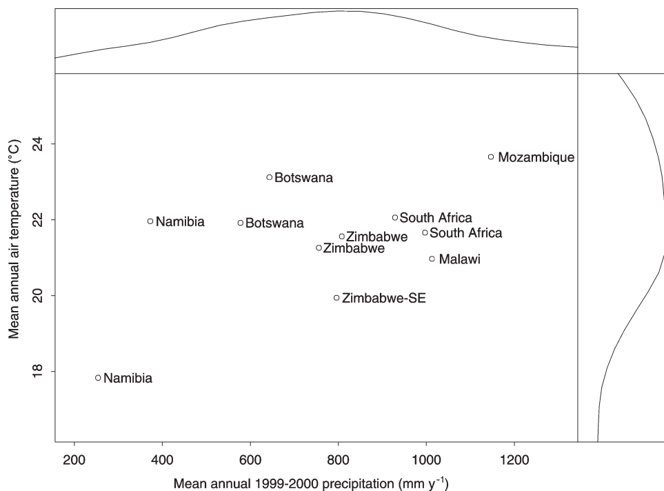
Figure 4. Mean annual air temperature (derived from 0.5^\circ mean monthly 2m air-temperature climatology data; Leemans and Kramer 1990) plotted against mean 1999 and 2000 annual precipitation (derived from the monthly 1^\circ Tropical Rainfall Measuring Mission best-estimate precipitation rate product; Huffman et al. 1995) at the geographic centres of the 11 Landsat ETM+ scenes illustrated in figures 2 and 3. Probability densities of the mean annual temperature and mean 1999 and 2000 annual precipitation for all of southern Africa (including Madagascar) are shown in the plot margins.
