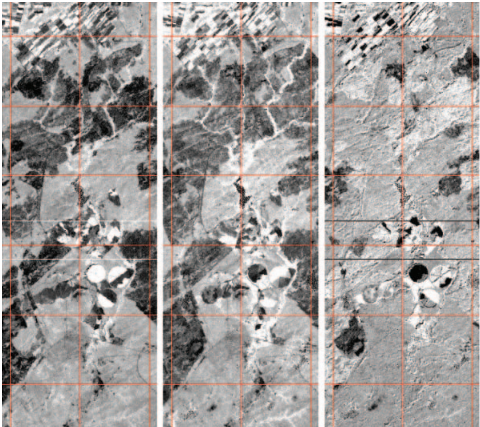
Figure 6. Spectral indices (\text{band } 5 - \text{band } 7)/(\text{band } 5 + \text{band } 7) computed for 10 September (left) and 12 October 2001 (middle) from the Landsat ETM+ data illustrated in figure 5. The right image shows the temporal difference of the spectral indices (12 October to 10 September).
