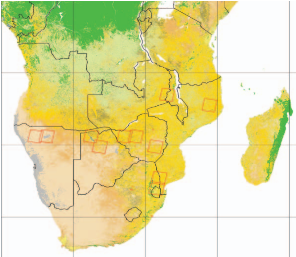
Figure 2. Eleven Landsat ETM+ validation scenes (red squares) superimposed upon MODIS 1 km land cover map (Friedl et al. 2002). Of the 17 MODIS land cover classes, predominant classes illustrated include: evergreen broadleaf forest (dark green), barren or sparsely vegetated (gray), woody savannas (light green), open shrublands (cream), grasslands (light brown), savannas (orange), croplands (yellow), cropland/natural vegetation mosaic (olive brown), urban (red). Country boundaries and meridians (10°, 20°, 30°, 40°, 50° East) and parallels (10°, 20°, 30° South) are shown (black lines).
