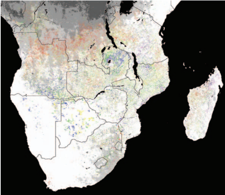
Figure 1. Temporal composite of the MODIS-Terra 1 km day and night active fire product over southern Africa, 1 March to 30 November (not including 10 June to 3 July) 2001. Fires occurring from March to the end of July (red), August (yellow), September (green), October (blue) and November (magenta). Black indicates water bodies. White and grey shades illustrate locations where no fires were detected and show the percentage of MODIS day and night 1 km observations labelled as cloudy by the MODIS active fire product over the 9 month period (white=0–10%, light grey=11–20%, grey=21–30%, dark grey=31–40%, some isolated pixels 41–50%). Country boundaries are shown (black lines).
