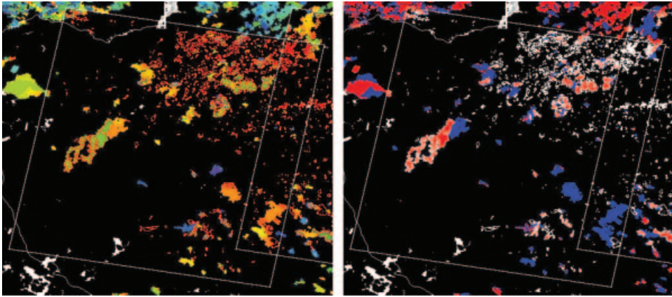
Figure 9. MODIS 500 m burned area product and Landsat ETM+ independent burned-area validation data, Matabeleland, Zimbabwe (Landsat Path 171, Row 73, the west Zimbabwe Landsat scene in figures 2 and 3). The vectors show independent burned-area data mapped using the protocol from two ETM+ acquisitions sensed 14 August and 1 October 2001 (left: red vectors; right: white vectors). Vectors for parts of the adjacent scene are also shown. The MODIS burned areas are coloured in the same way as figure 7. The 185 \times 170 km Landsat ETM+ scene boundary and the Botswana and Zambian boundaries are also shown (white vectors, left and right).
