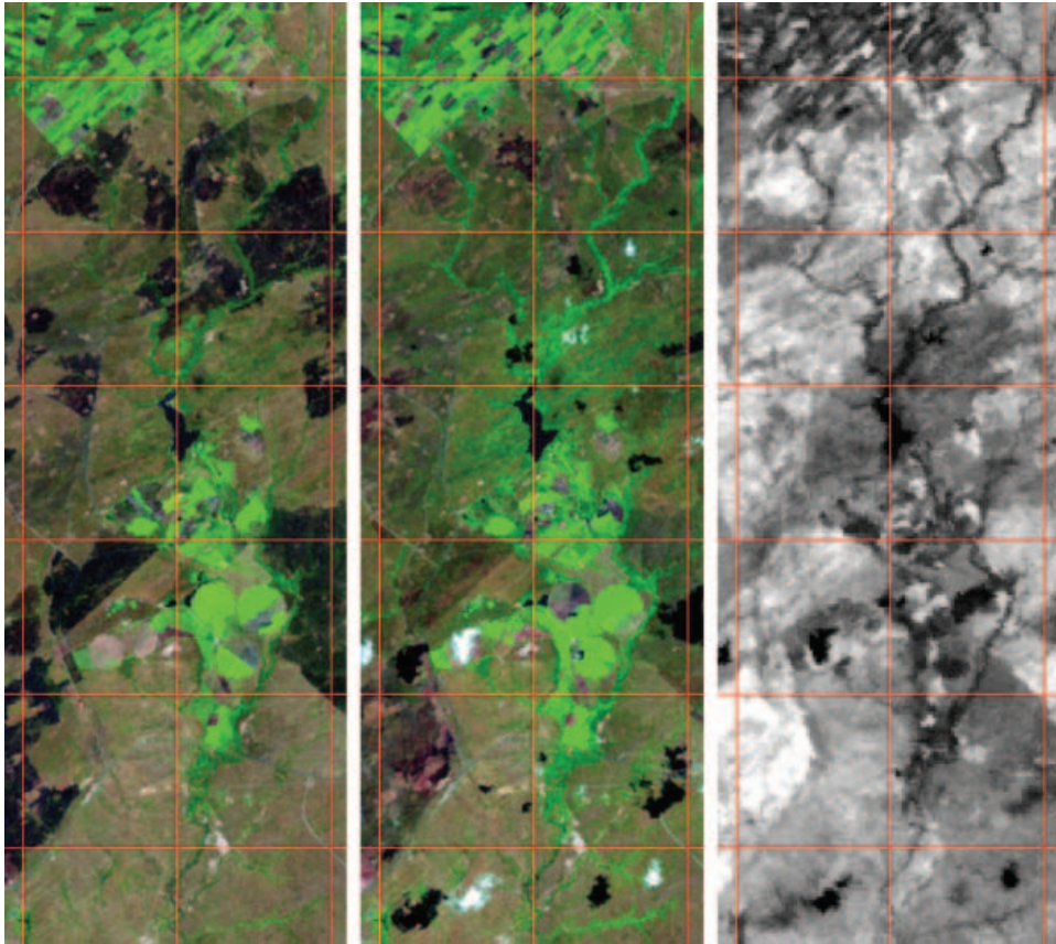
Figure 5. Landsat ETM+ 30 m reflective wavelength data acquired 10 September (left) and 12 October (middle), and 60 m thermal wavelength data acquired 12 October (right), 2001, near the Save Valley Conservancy, Zimbabwe (the south-east Zimbabwe Landsat scene illustrated in figures 2–4). Reflective 30 m data displayed as red: band 5 (1550–1750 nm), green: band 4 (750–900 nm), blue: band 3 (630–690 nm). Thermal 60 m band 6 (10.4–12.5 \mu\text{m} ) data displayed as a greyscale (lighter tones are warmer). The red grid lines are spaced every 3 km. The water body in the image centre is located at 20^{\circ} 55' 15''\text{S} , 31^{\circ} 47' 37''\text{E} . Burned areas appear dark in the reflective wavelength data and light in the thermal data. Clouds and cloud shadows are evident across the 12 October data.
