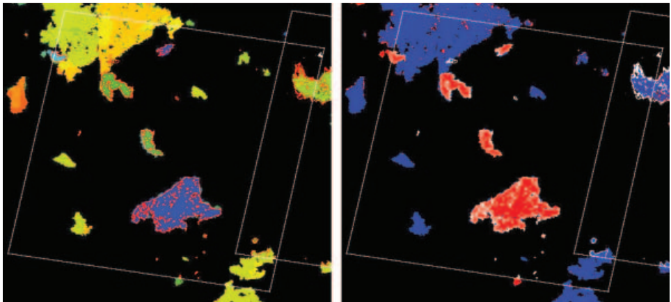
Figure 7. MODIS 500 m burned-area product coloured pixels and Landsat ETM+ independent burned-area validation data vectors, Namibia (Landsat Path 180, Row 73, the west Namibian Landsat scene in figures 2 and 3). The vectors show independent burned-area data mapped using the protocol from two ETM+ acquisitions sensed 6 August and 23 September 2001 (left: red vectors; right: white vectors). Vectors for parts of the adjacent scene are also shown. The coloured pixels show the burned areas detected by MODIS over 105 days from 20 July to 1 November 2001 (left: coloured with a rainbow scale to indicate the approximate day of burning; right: red to indicate burned areas detected within the Landsat ETM+ acquisition period, blue to indicate MODIS burned areas detected before or after the ETM+ acquisition period). Black indicates no burning detected by MODIS. White pixels show areas that could not be mapped due to missing MODIS data or persistent cloud. The 185 \times 170 km Landsat ETM+ scene boundary is shown (white box).
