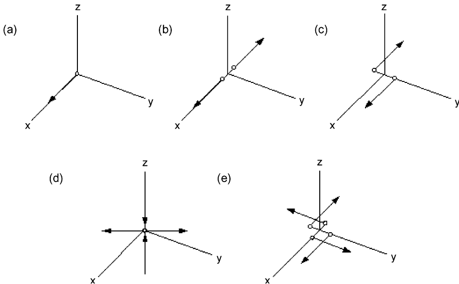
Fig. 1. Various force types at a point source: (a) a single force; (b) a pair of equal and opposite forces in tension; (c) a pair of equal and opposite forces as a torque about the z-axis; (d) two pairs of forces, where tension and compression are of equal magnitude and are perpendicular to one another; (e) two pairs of forces with torques about the z-axis of equal magnitude and opposite in direction (redrawn from Kasahara, 1981)
