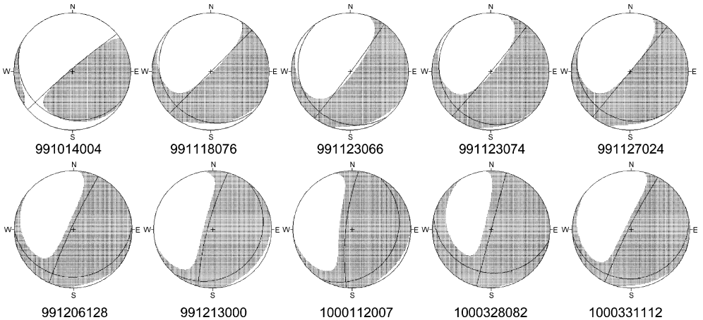
Fig. 9. Radiation patterns and fault-plane solutions for the cluster computed with the hybrid MTI using a median correction (Scheme B)
