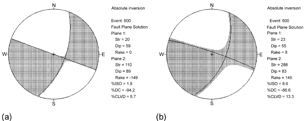
Fig. 2. Radiation patterns and source parameters computed from synthetic data using the absolute MTI technique. (a) Noise free case. (b) 40% random noise applied to all channels
