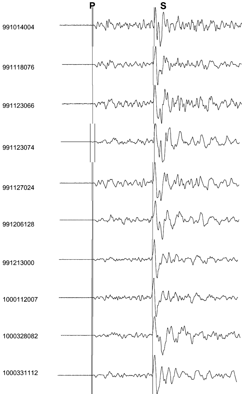
Fig. 6. Velocity waveforms plotted using the same time axis as recorded by site 1, component 2. Note similarity of waveforms. P-wave onset and S-wave onset are marked 'P' and 'S' respectively
