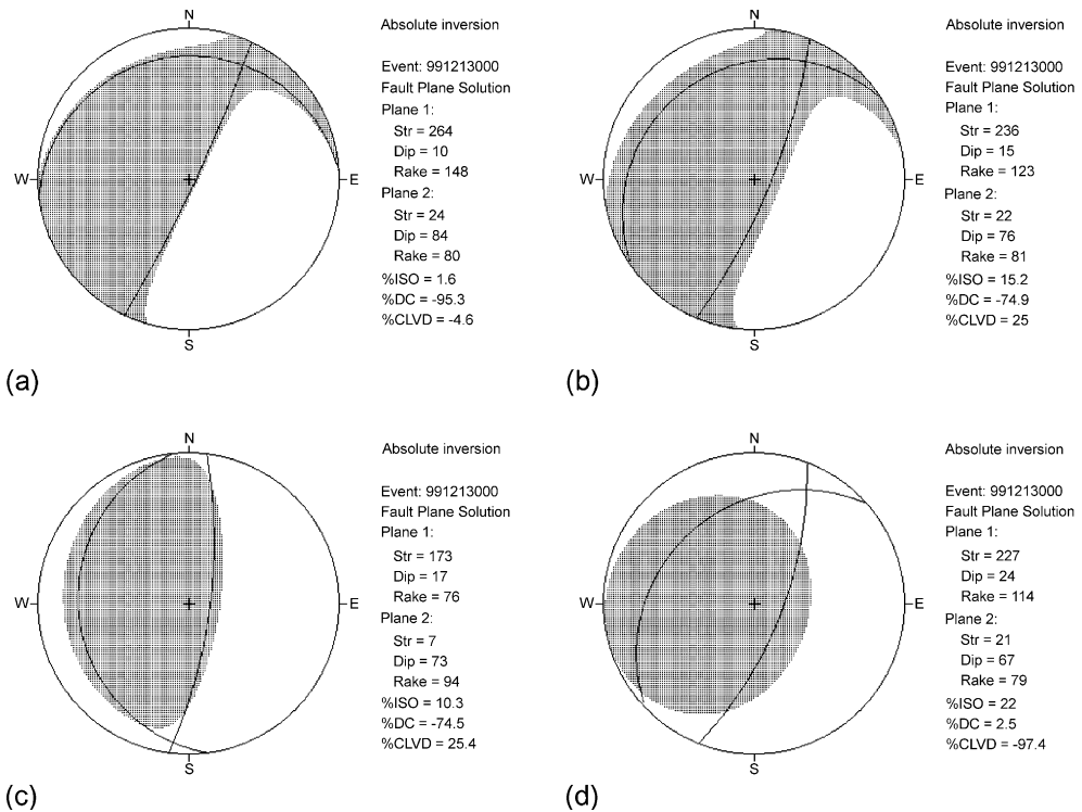
Fig. 3. Radiation patterns and source parameters computed from recorded data using the absolute MTI method (a) Control case, (b) 40% random noise applied to all channels, (c) reversed P- and S-wave polarities for site 1, and, (d) bad phase picks for P- and S-wave for site 1, component 1
