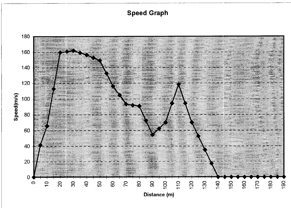
Figure 4.4.1b: Test 96: 80 bags
