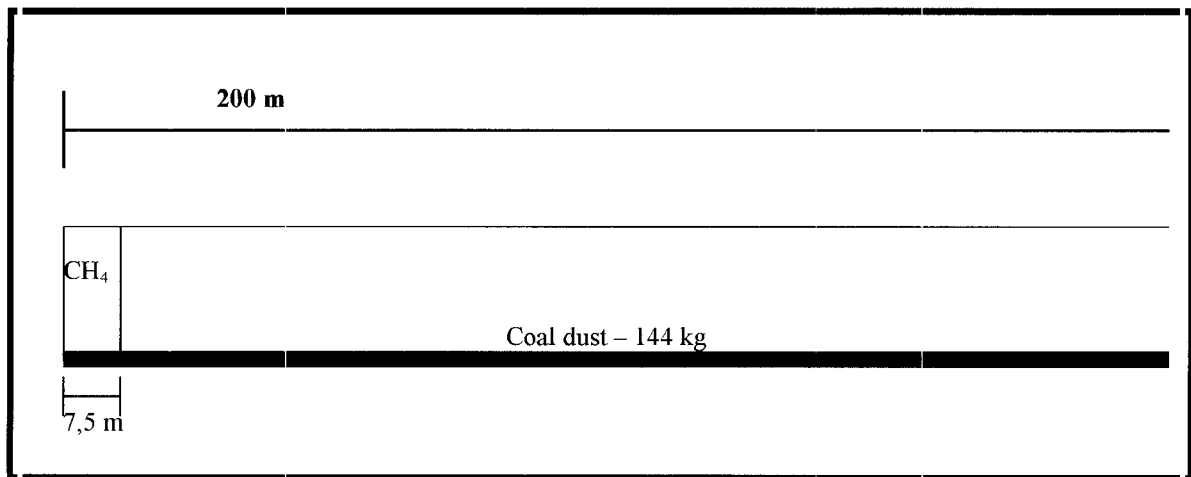
Figure 4.1.1: Test layout for the standard explosion
