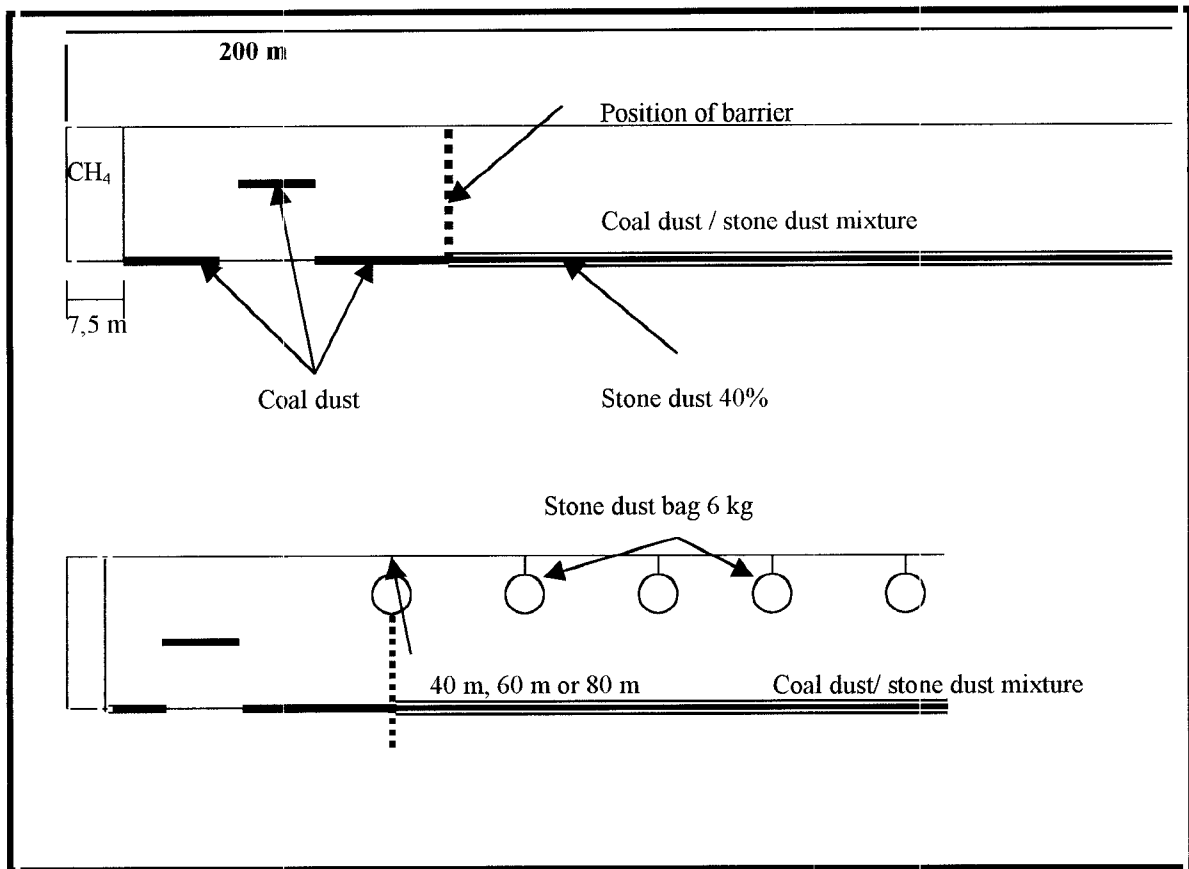
Figure 4.1.5: Test layout for the supplement explosions
