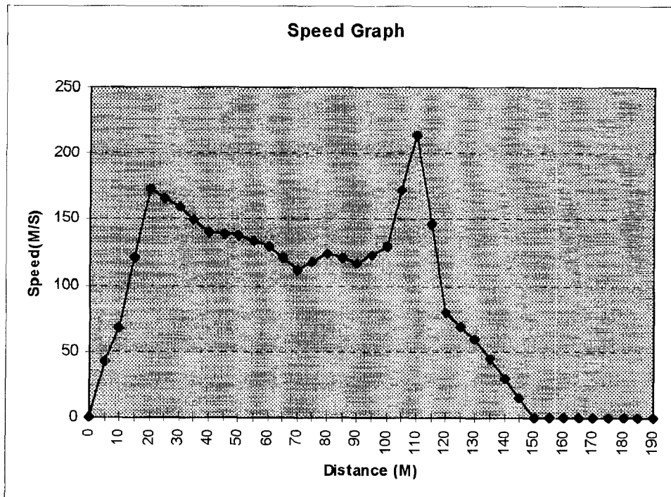
Figure 4.4.2: Explosion 86: 60 bags
