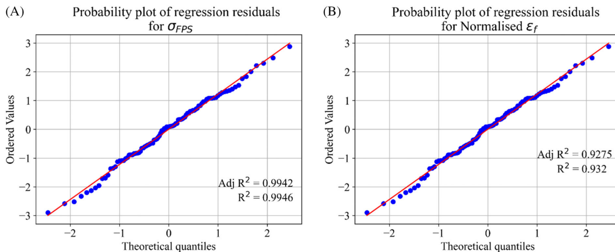
FIGURE 5 Probability plot of the residuals for (A) \sigma_{FPS} and (B) normalized \varepsilon_f .
