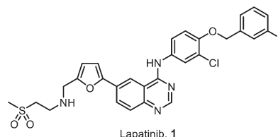
Fig. 1 Structure of lapatinib, 1 .
