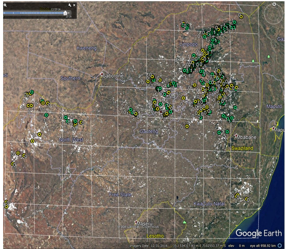
Fig. 2. Validation of increasing tree cover map using Google Earth imagery. 1green = evidence of increasing tree-cover and 0 yellow = no evidence of change in tree cover. White polygons denote areas with a significant p < 0.05 increasing trend in tree-cover.
