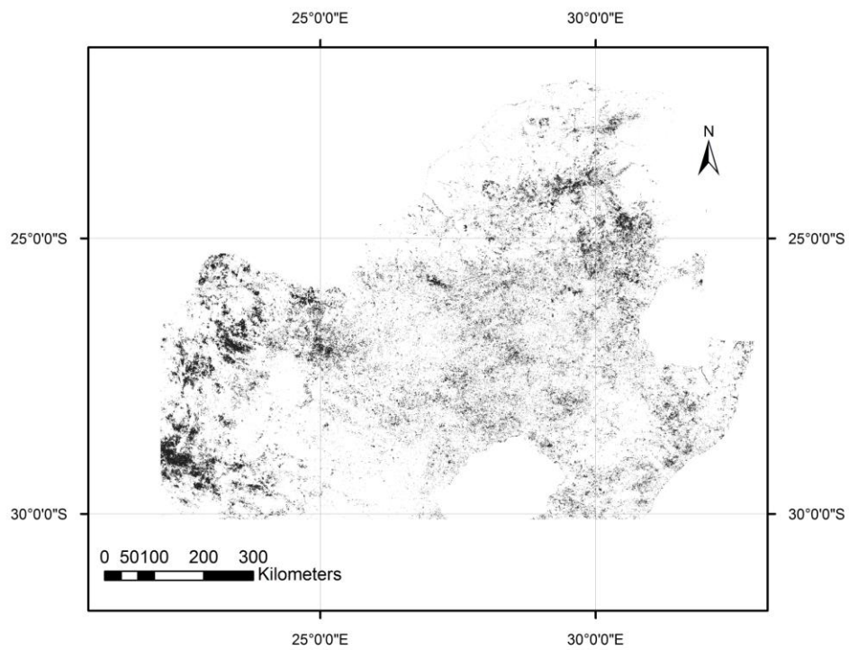
Figure 9. Areas of significant p < 0.05 increasing or decreasing trend in NDVI derived from Kendall correlation analysis.
