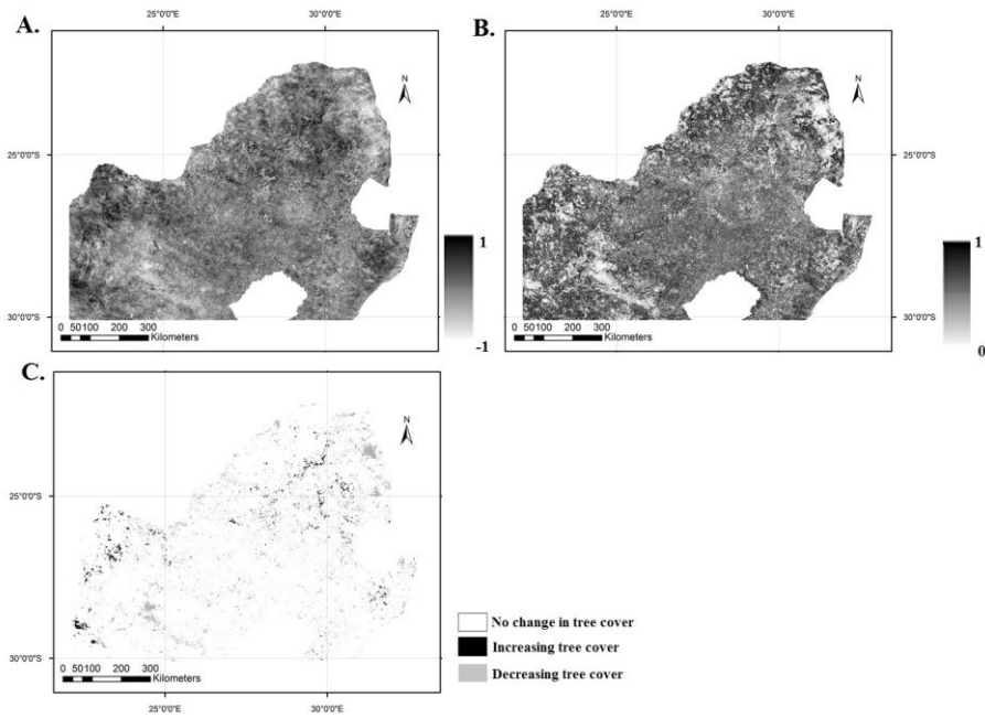
Fig.5. Trend analysis of tree-cover change 2001 – 2018 using Kendall correlation analysis. A = Kendall Tau coefficient, B = p -values and C = threshold of p < 0.05 highlighting the areas of significant increasing or decreasing tree-cover percentage.
