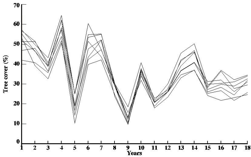
Figure 7. Tree-cover profiles of an area in the Kruger National Park that showed significant decreasing trend in tree-cover between 2001 and 2018. The area was burnt in the winter of 2008.
