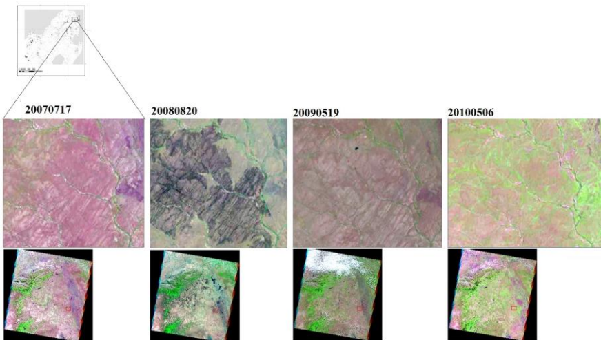
Figure 8. Landsat TM5images 2007, 2008, 2009 and 2010 of an area in the Kruger National Park that showed significant decreasing trend in tree-cover between 2001 and 2018. A fire scar can be observed in 2008.
