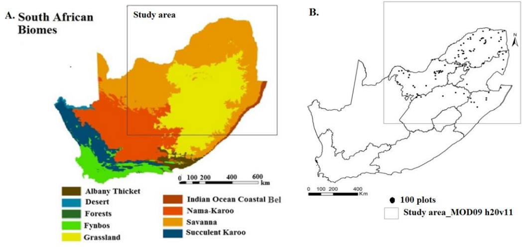
Fig. 1. Fig.1. Biomes of South Africa A Mucina and Rutherford, 2006 and 100 random plots selected to analyse the relationship between NDVI and percentage tree cover B.
