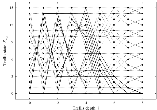
Fig. 5. Unexpurgated (dotted branches) and expurgated (solid branches) trellis structure of the RM(8, 4, 4) code
