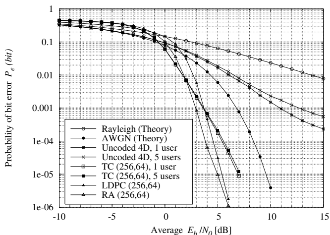
Fig. 10. Multipath performance comparison of (256,64) coding schemes
