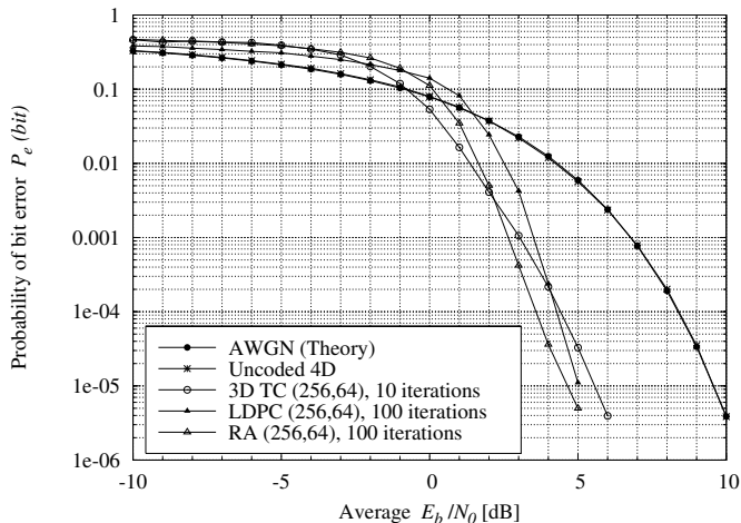
Fig. 9. AWGN performance comparison of (256,64) coding schemes
