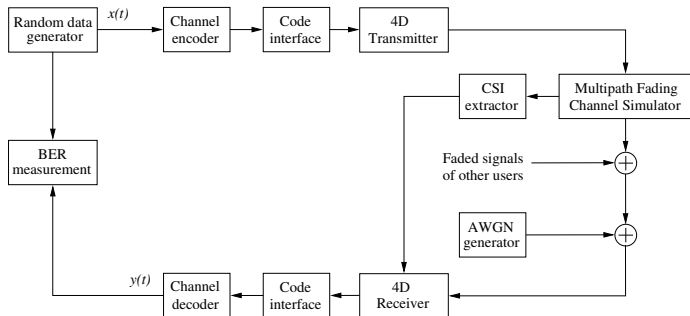
Fig. 6. Coded simulation platform
