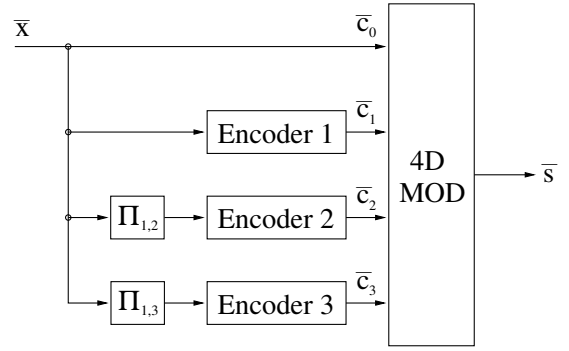
Fig. 3. Encoder and 4D modulator structure
