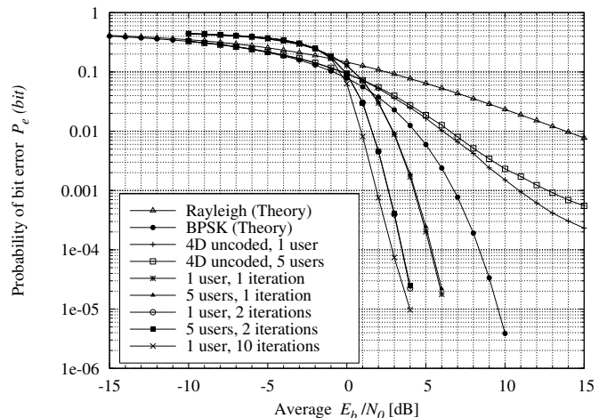
Fig. 8. Multipath fading performance results for 1 to 5 CDMA users
