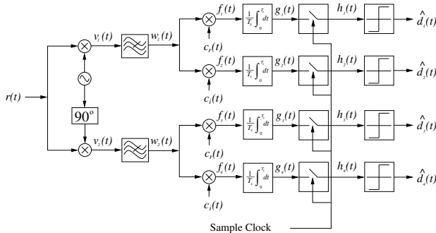
Fig. 2. Four dimensional DSSS receiver structure
