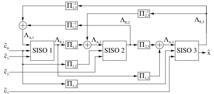
Fig. 4. Three-dimensional block turbo decoder structure
