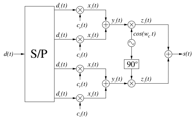
Fig. 1. Four dimensional DSSS transmitter structure
