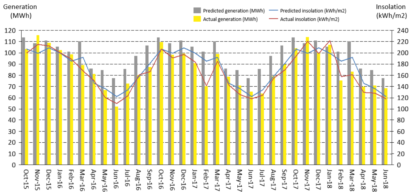
Figure 2 : Single axis tracker insolation and generation (predicted vs actual)
