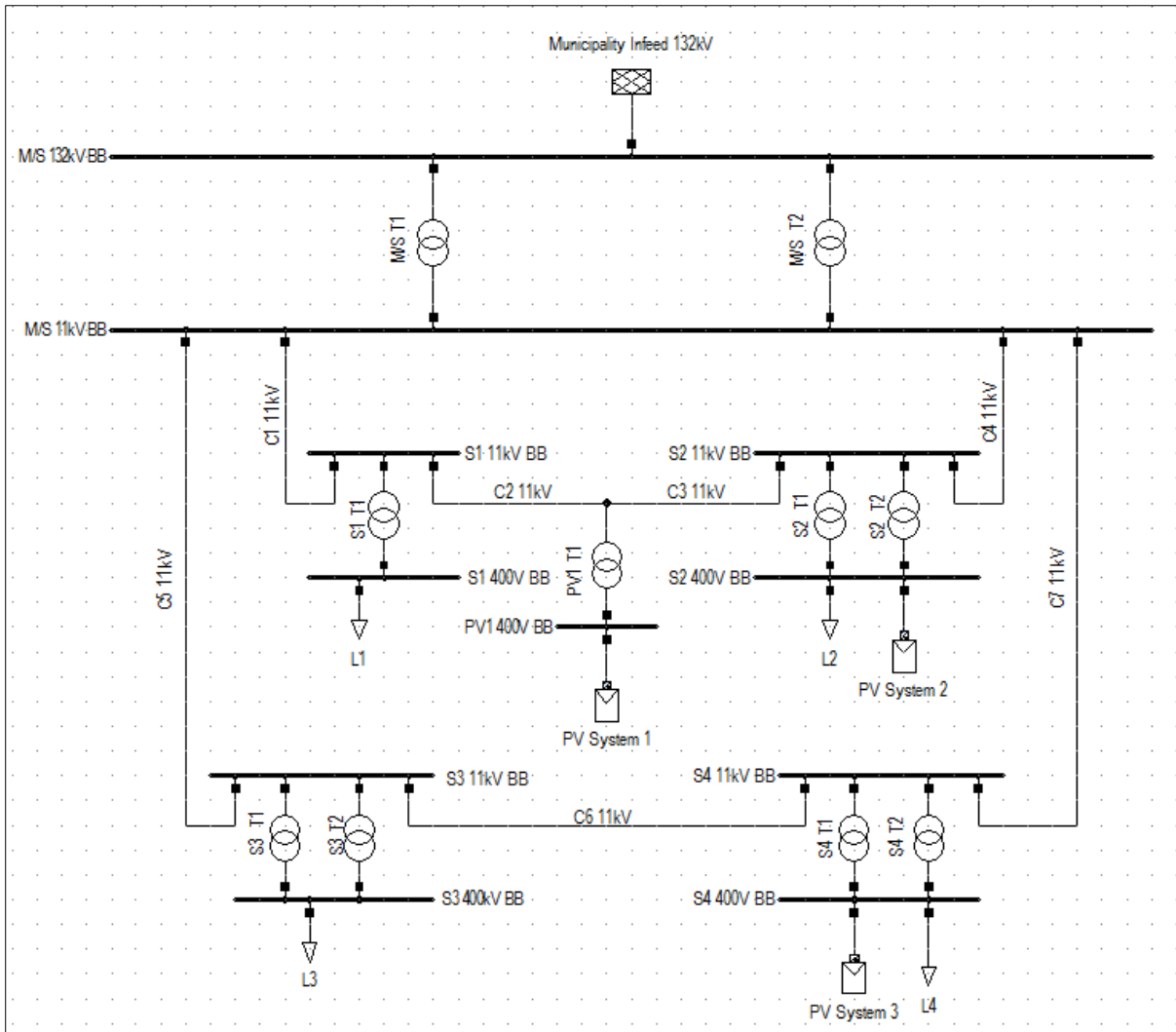
Figure 1: The single line diagram of the three PV systems connected at MV and LV levels
