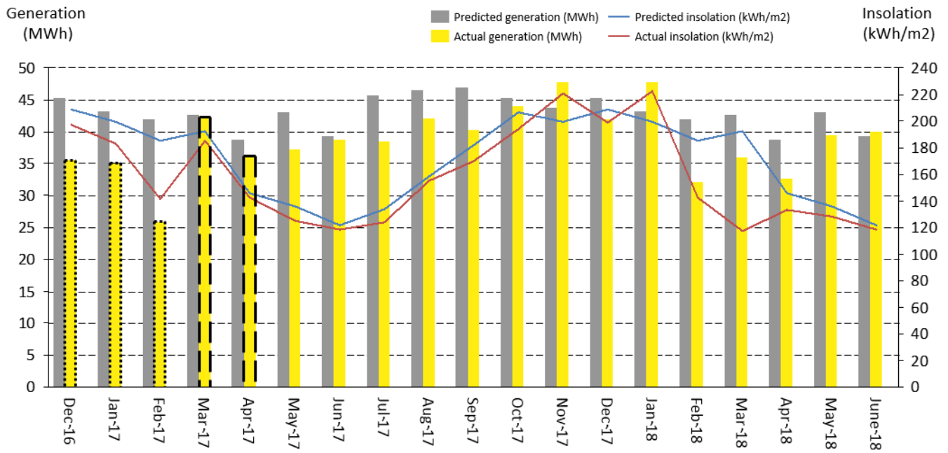
Figure 3: Dual axis tracker insolation and generation (predicted vs actual)
