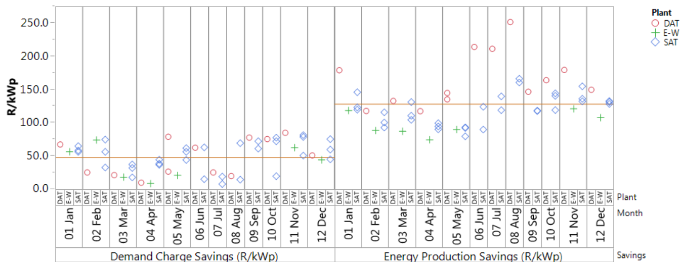
Figure 10: Monthly savings per kWp from maximum demand and energy consumption reduction by each plant
