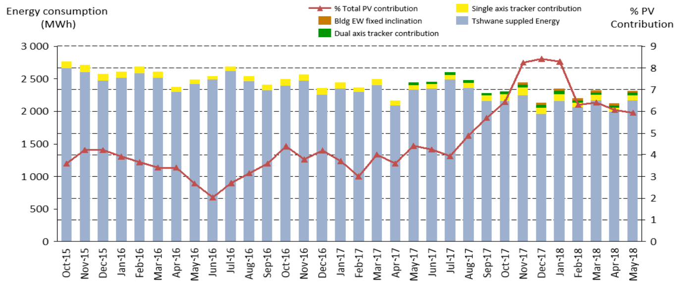
Figure 5: Solar PV monthly contribution towards organisation's total energy consumption
