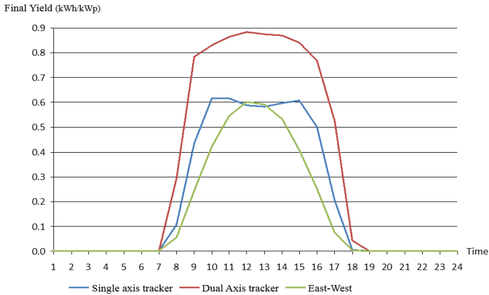
Figure 8: Final yield on a typical winter day (2 June 2018)
