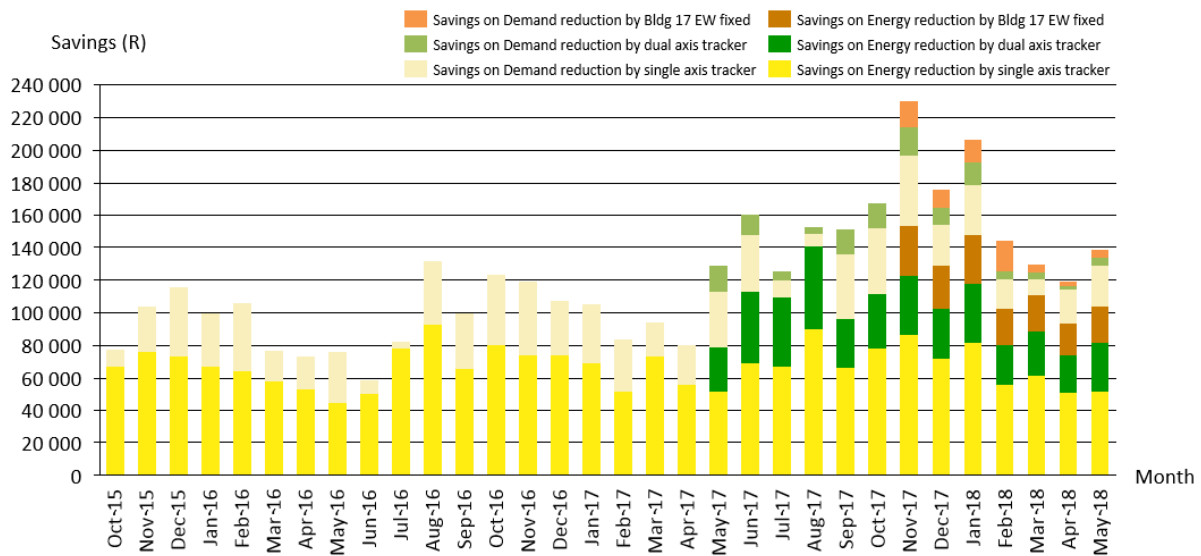
Figure 9: Monthly savings on maximum demand and energy consumption reduction by each plant
