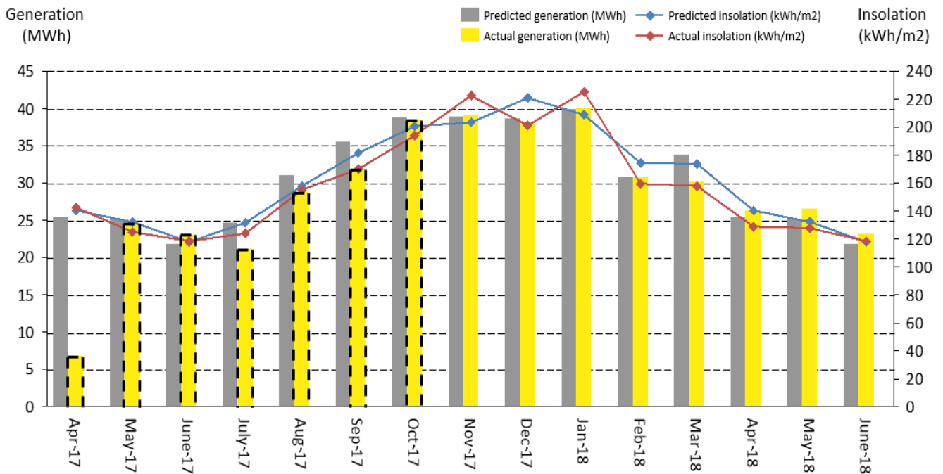
Figure 4: East-west fixed system insolation and generation (predicted vs actual)
