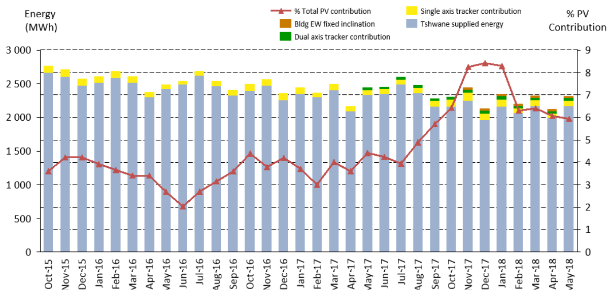
Figure 6: Solar PV monthly contribution towards organisation's maximum demand reduction
