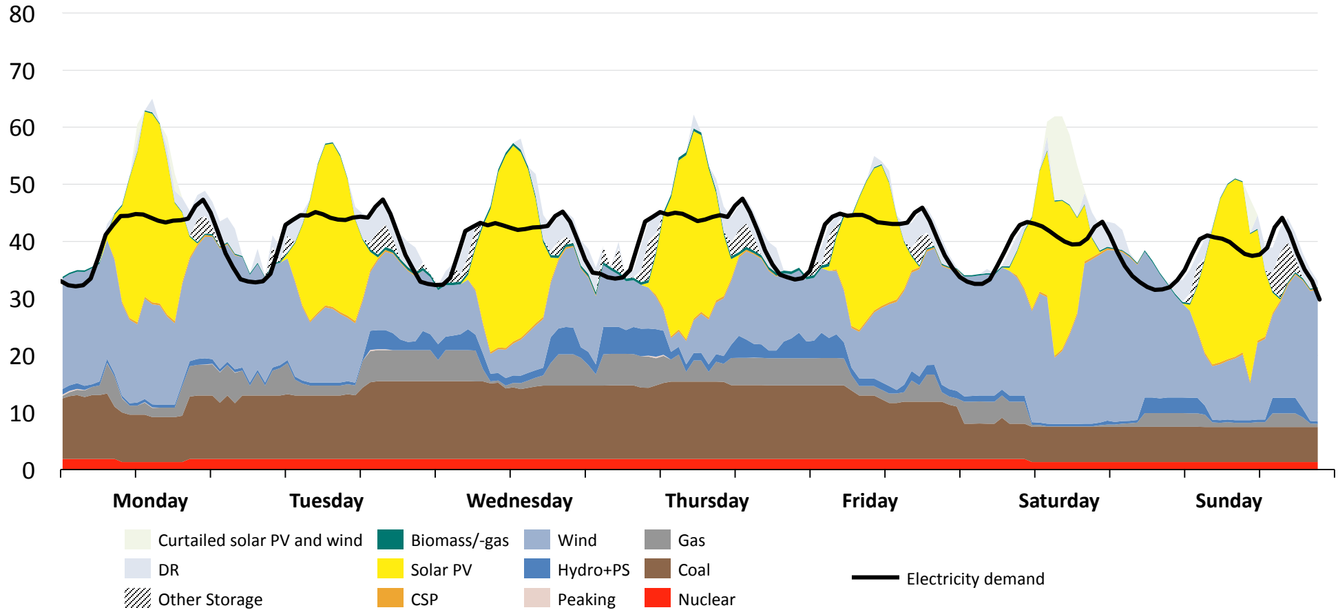
Exemplary Week under Risk-Adjusted Scenario
