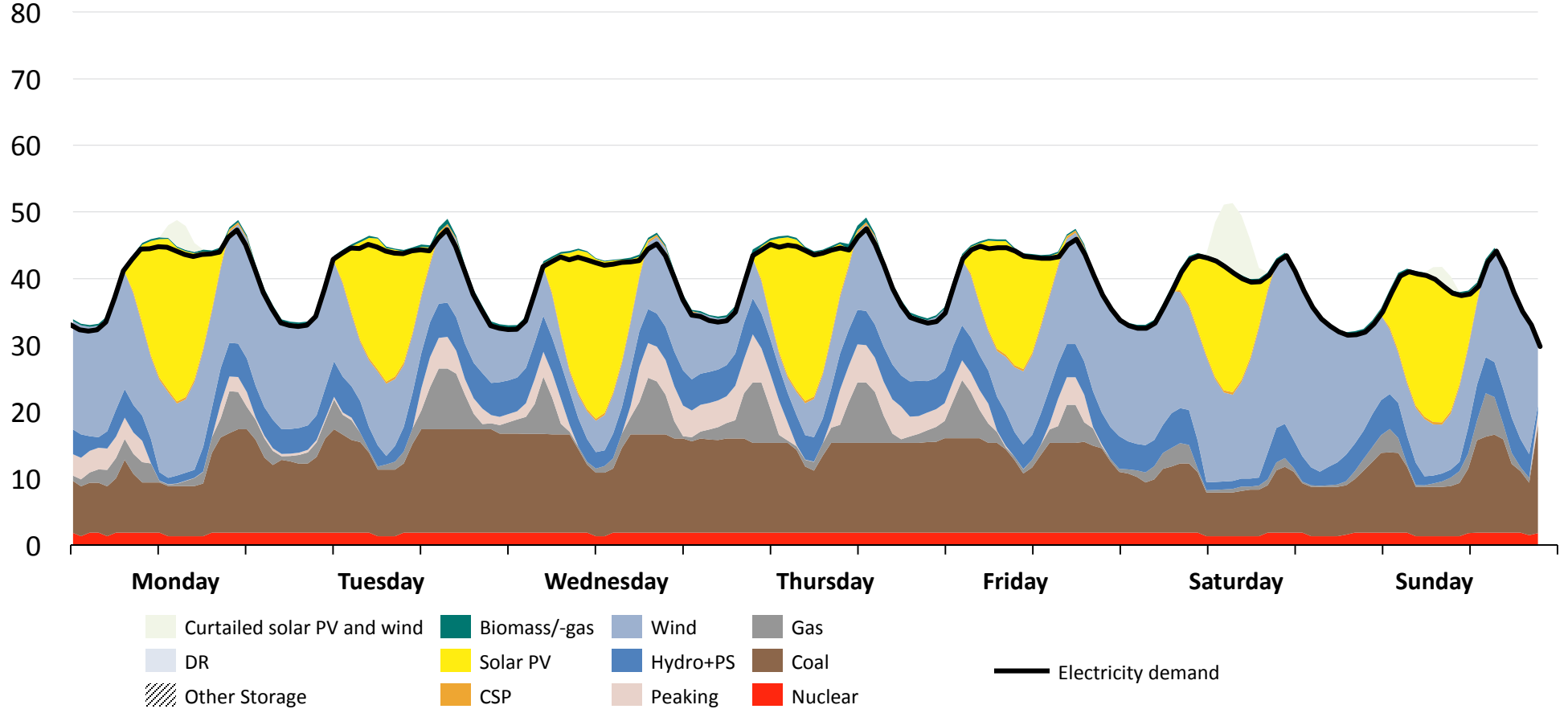
Exemplary Week under Draft IRP 2018 IRP1
