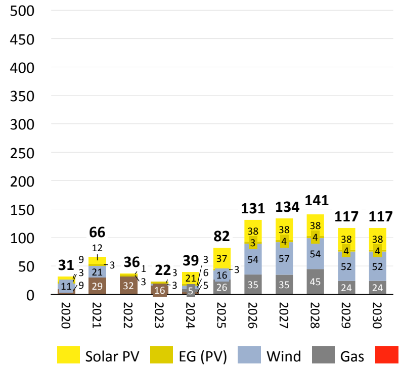
Construction jobs ['000]
