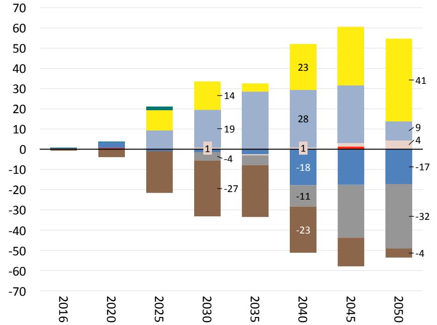
Difference - Electricity production [TWh/yr]
