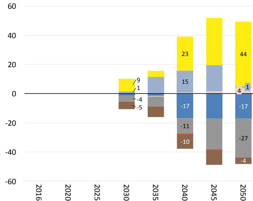
Difference - Electricity production [TWh/yr]
