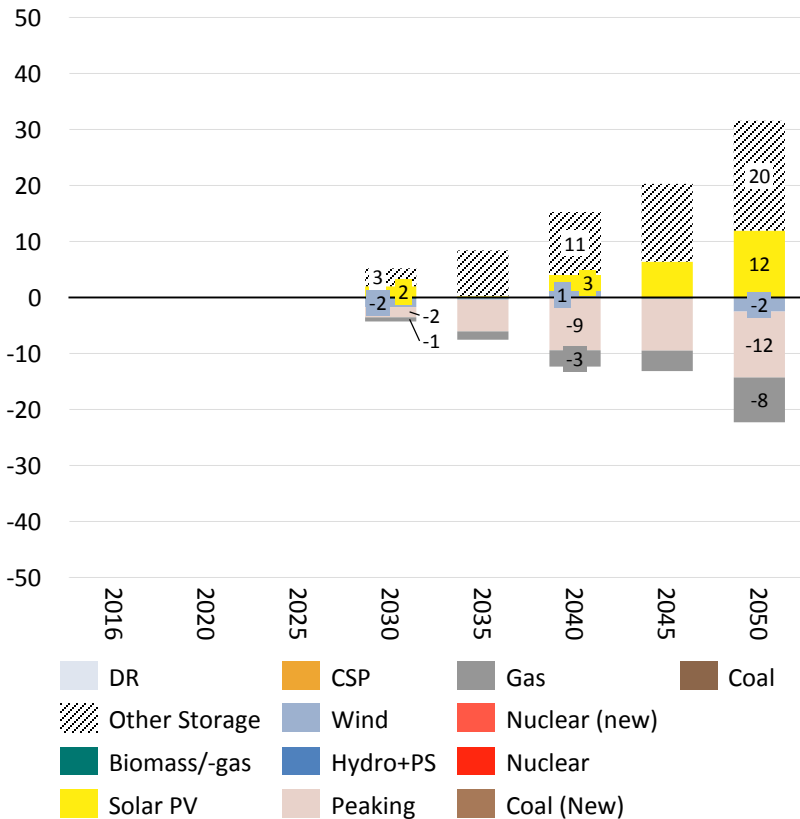
Difference - Total installed capacity (net) [GW]
