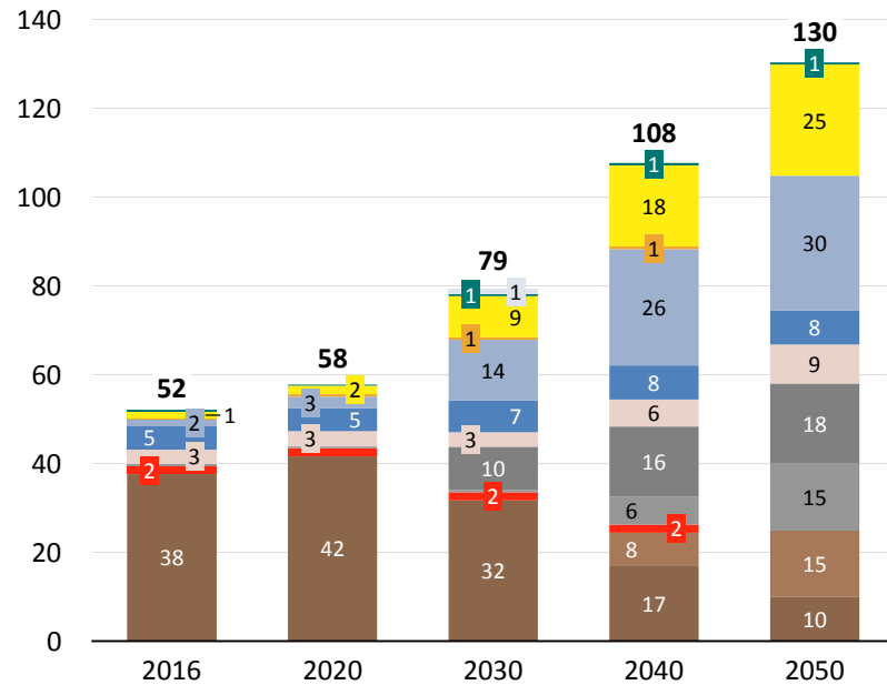
Total installed capacity (net) [GW]
