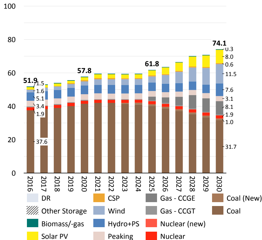
Total installed capacity (net) [GW]
