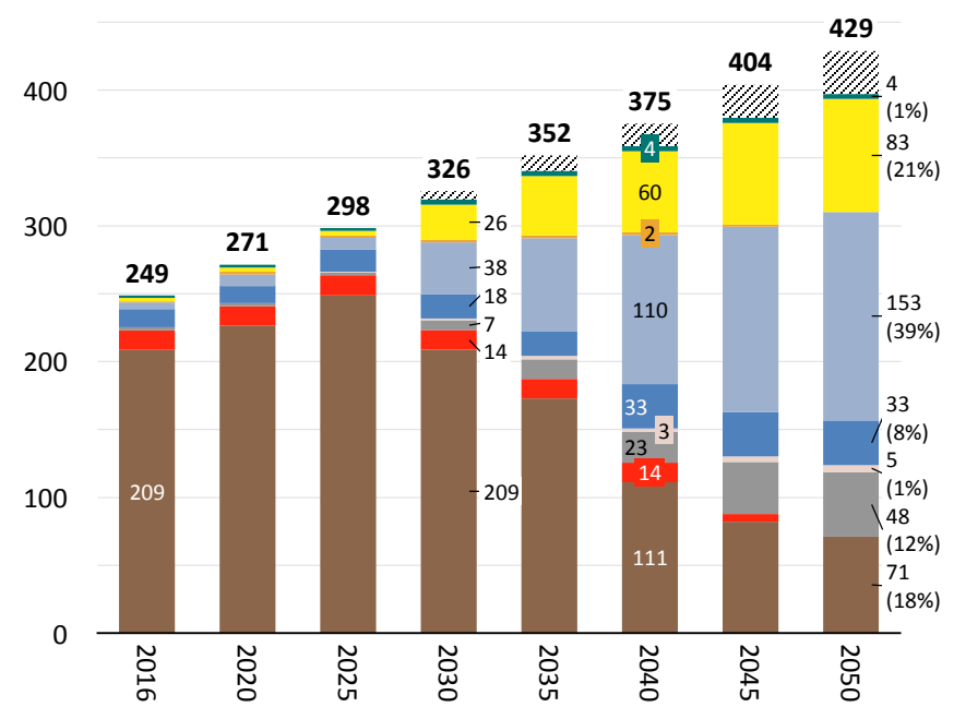
Electricity production [TWh/yr]
