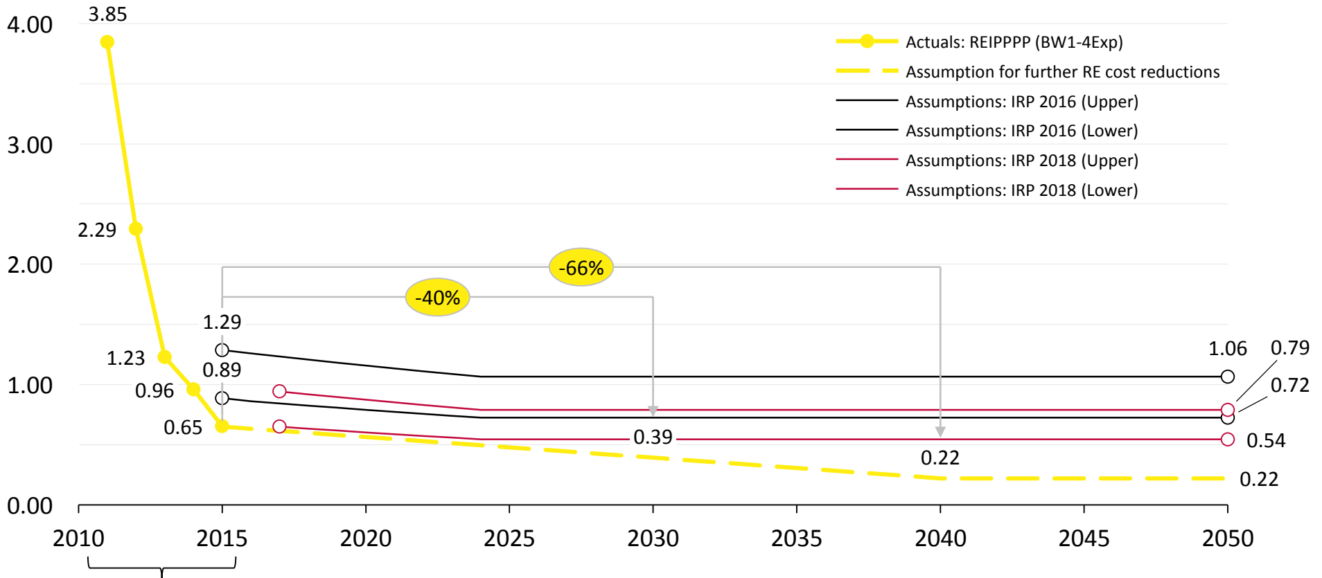
Equivalent tariff, Jan 2017, [ZAR/kWh]
