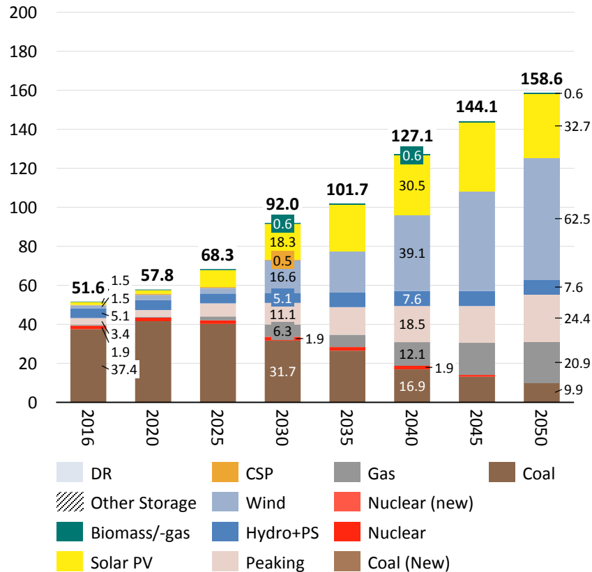
Total installed capacity (net) [GW]
