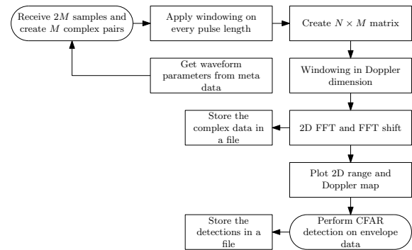
Fig. 8. The signal processing algorithm.
