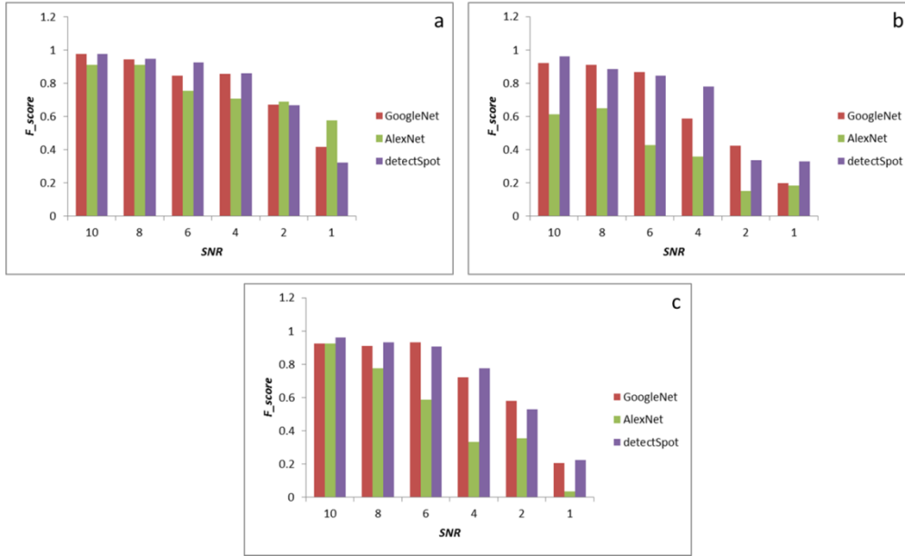
Fig. 5. F\_score vs SNR curves for all three conv-nets methods applied to two kinds of synthetic images (a) Synthetic type A, and (b-c) Synthetic type B.
