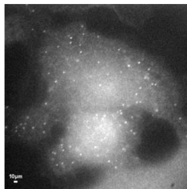
Fig. 1. A sample of real fluorescence image with bright particles obtained using confocal microscopy.
