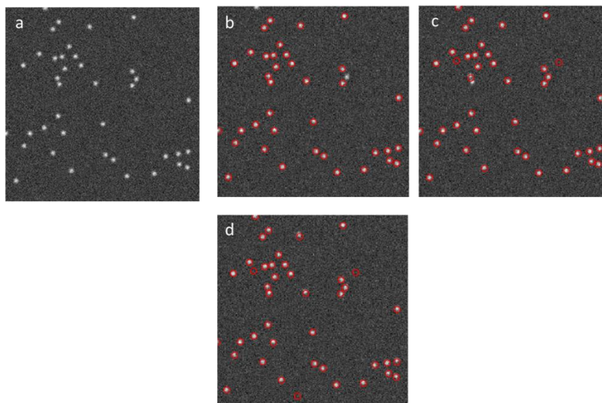
Fig. 6. Results of applying the proposed conv-nets methods on a synthetic image data. Detected spots by each method are showed in red circles.(a) Original synthetic image. (b) Spots detected by our approach, detectSpot. (c) Detected spots using GoogleNet. (d) Detected spots with AlexNet.
