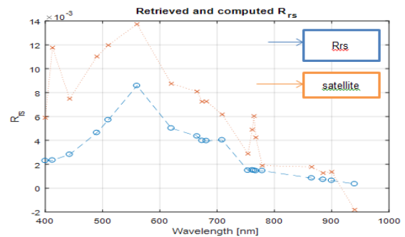
Fig.11 Retrieved Remote sensing reflectance of water leaving radiance versus Retrieved Sentinel3 data. That is possible be of the adjacency effect, the sentinel 3 picked up signal but the Rrs shows absorption.
